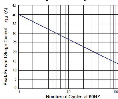
Figure 6: Maximum Non-Repetitive Forward Surge Current Only Unidirectional
