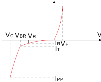
FIG.1:V- I curve characteristics (Uni-directional)
