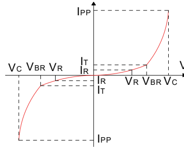
FIG.2:V- I curve characteristics (Bi-directional)
