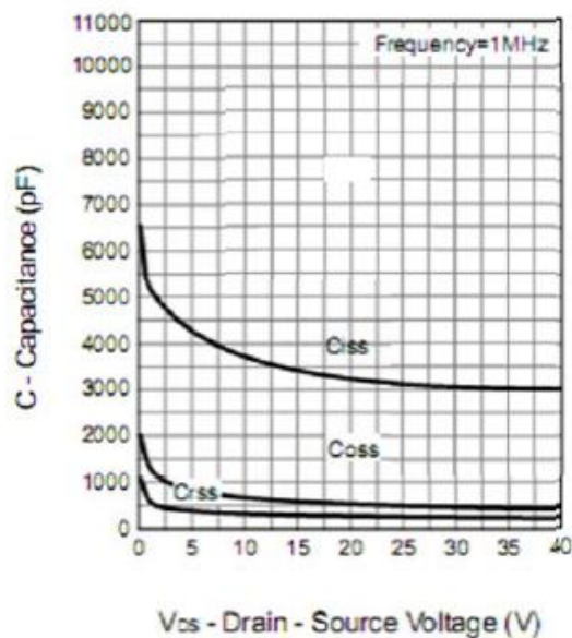
Capacitance
