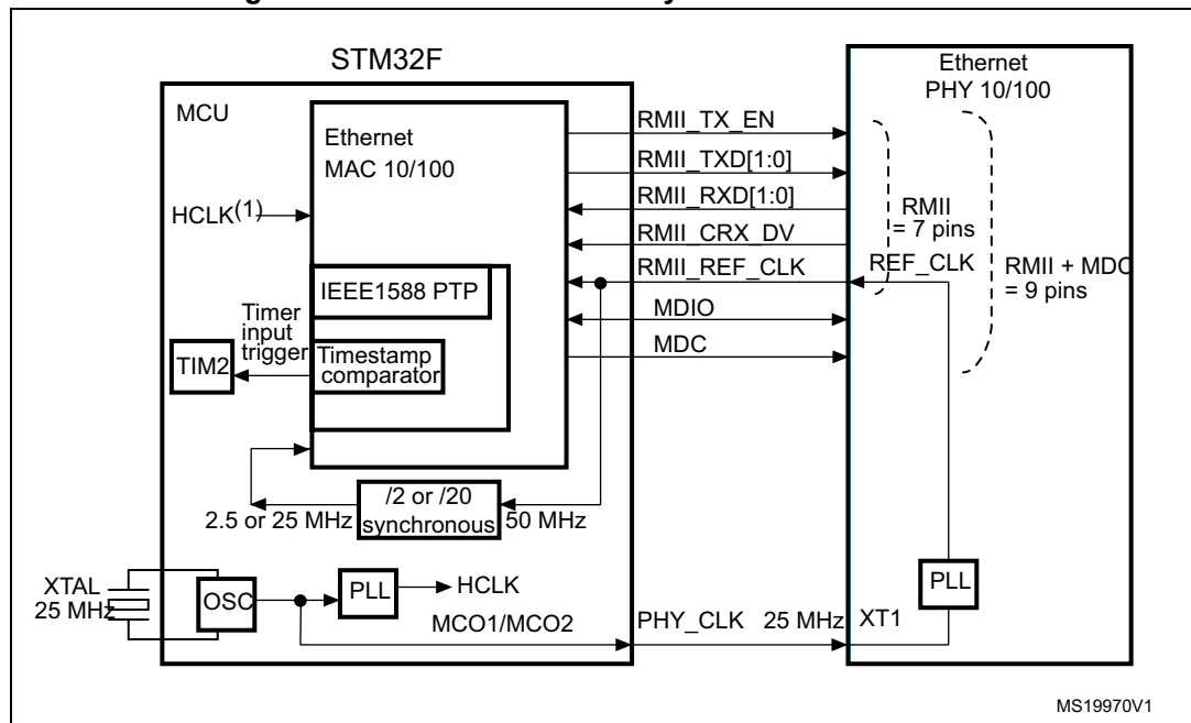
Figure 91. RMII with a 25 MHz crystal and PHY with PLL
