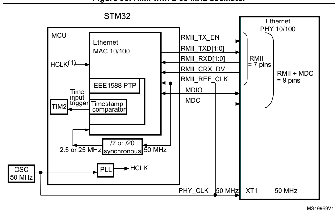
Figure 90. RMI with a 50 MHz oscillator
