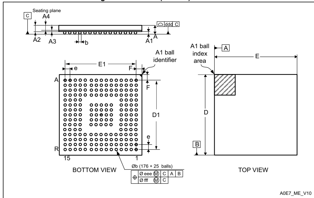
Figure 81. UFBGA(176+25) - Outline
