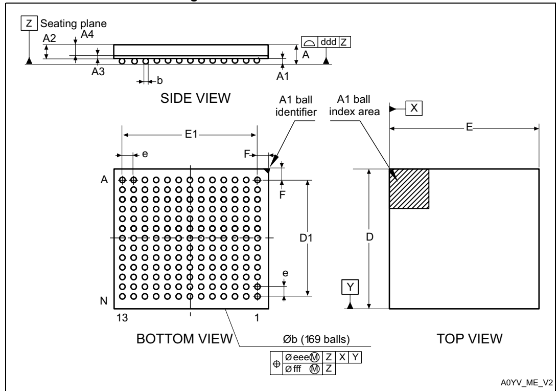
Figure 104. UFBGA169 - Outline
