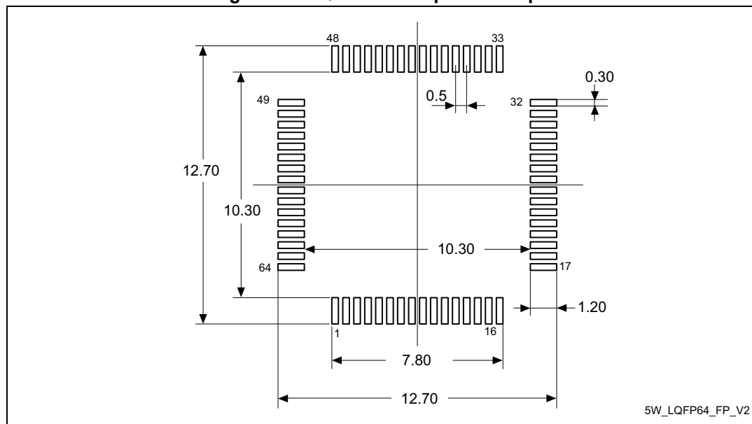
Figure 90. LQFP64 - Footprint example
