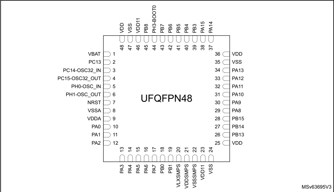
Figure 9. UFQFPN48_SMPS pinout
