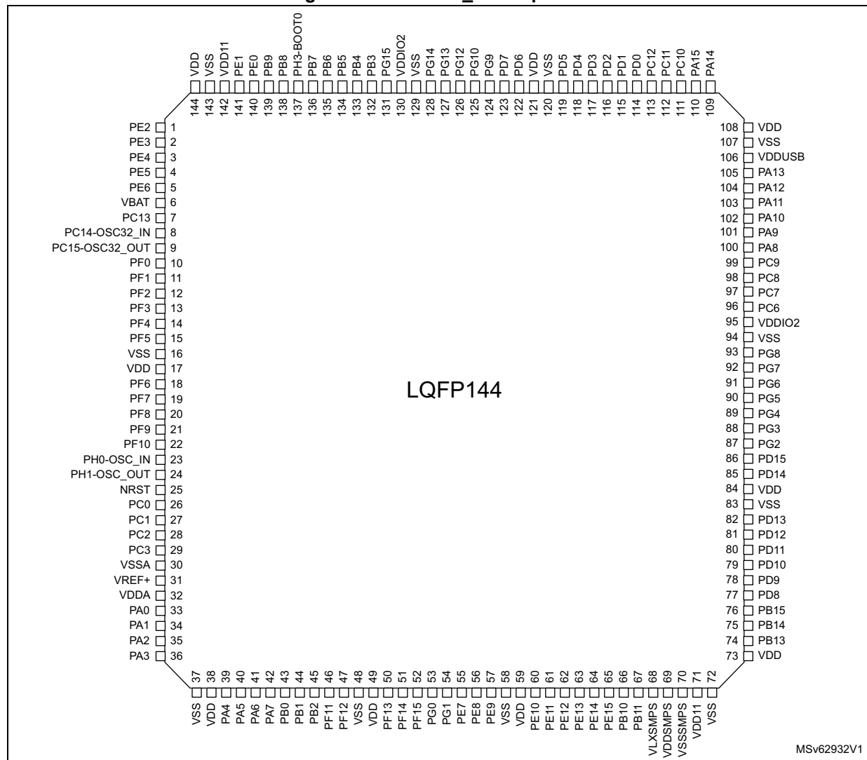
Figure 18. LQFP144_SMPS pinout
