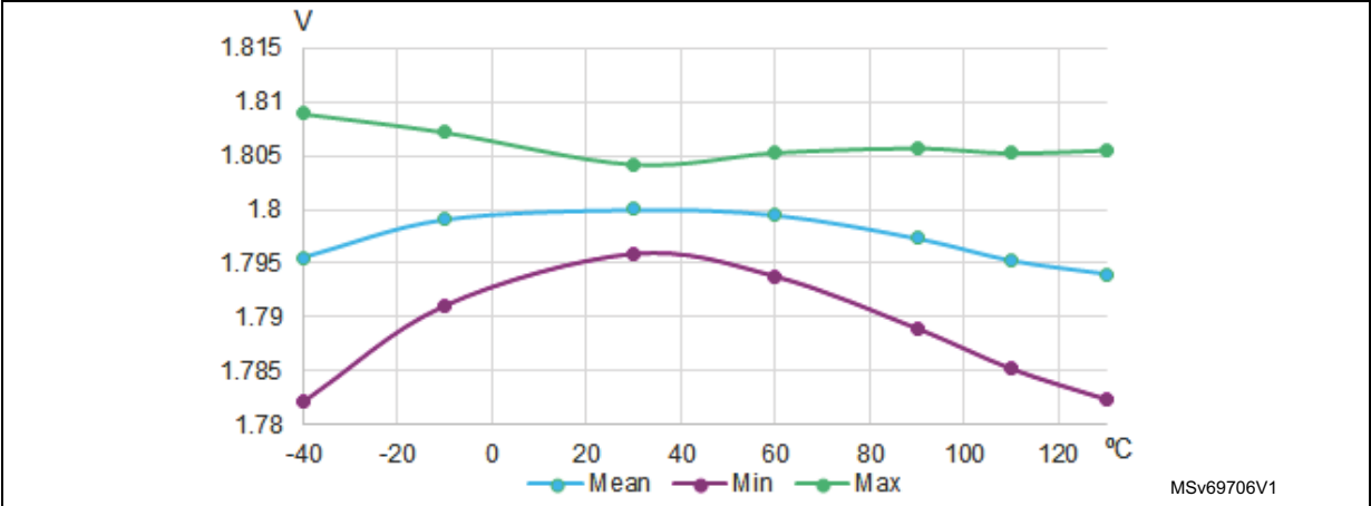
Figure 43. V_{\text{REFBUF OUT}} versus temperature (VRS = 001)
