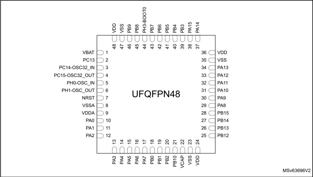
Figure 10. UFQFPN48 pinout
