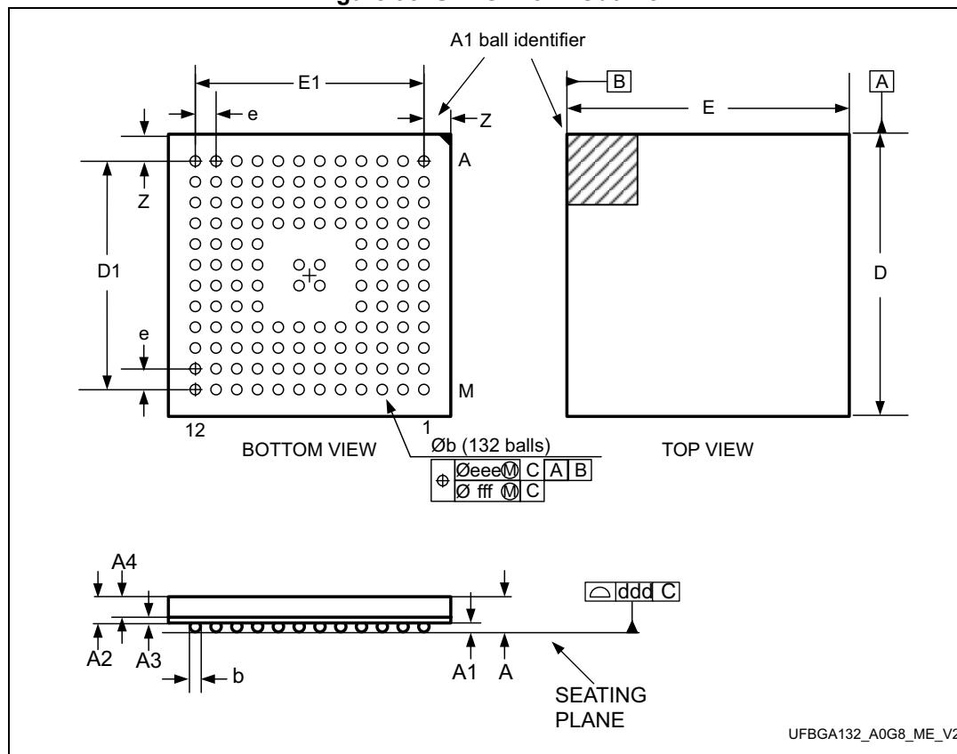
Figure 98. UFBGA132 - Outline
