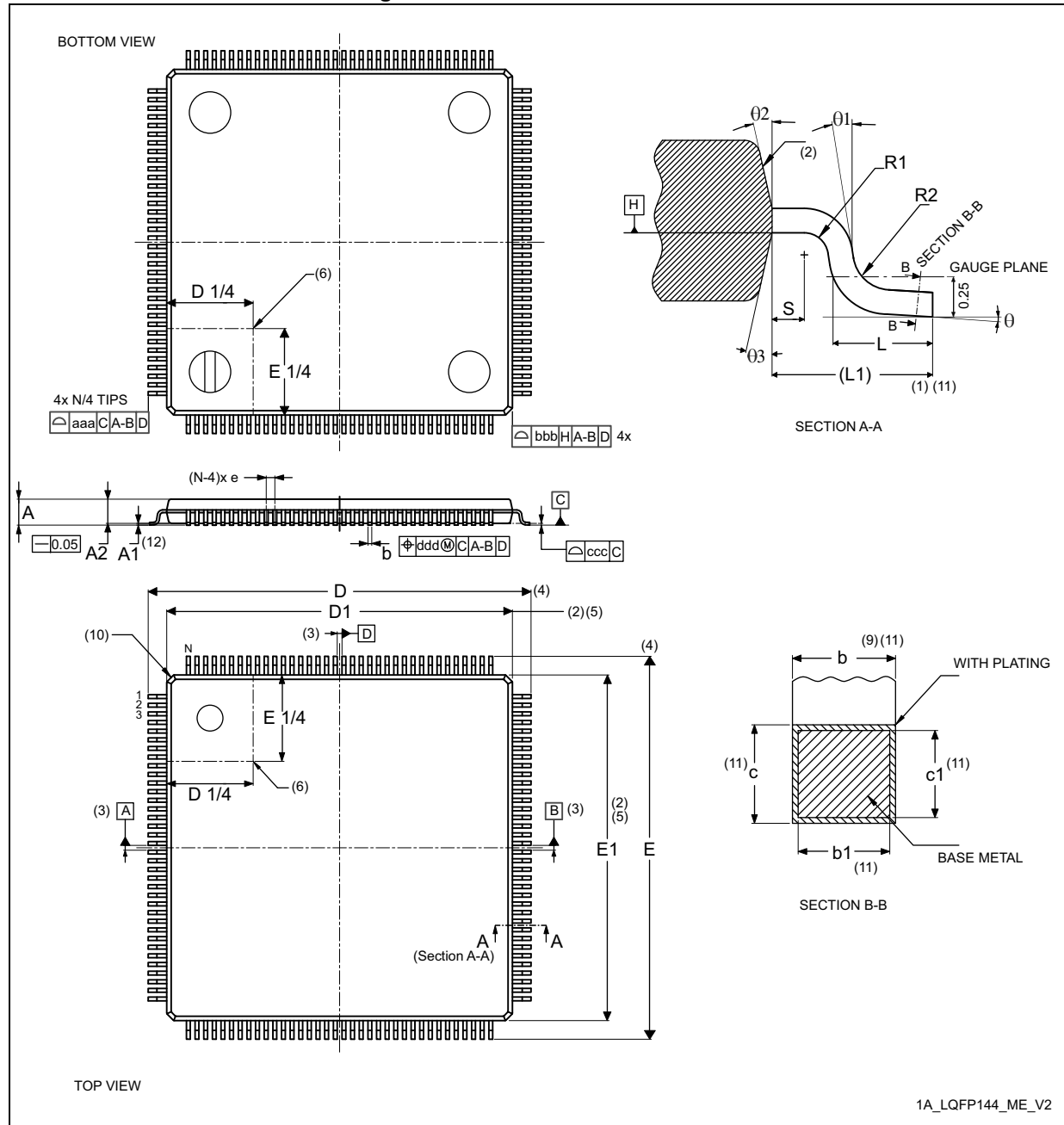
Figure 101. LQFP144 - Outline (15)
