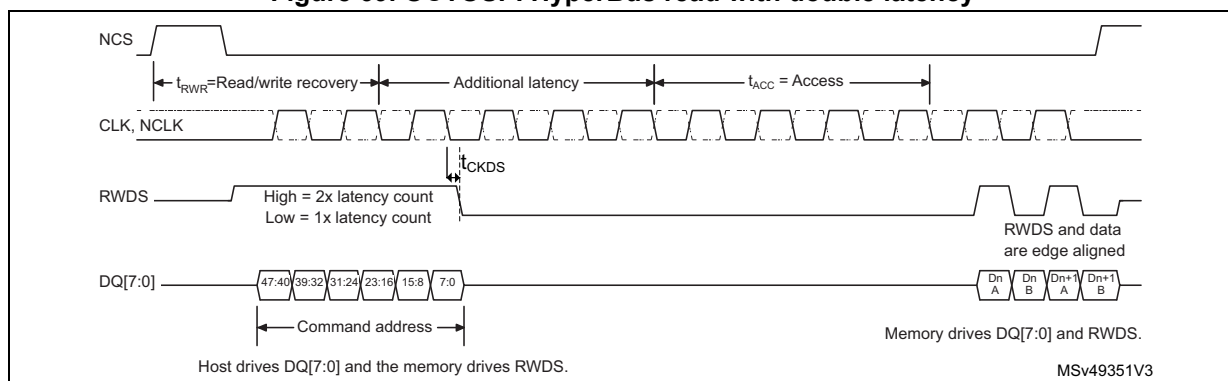
Figure 69. OCTOSPI HyperBus read with double latency
