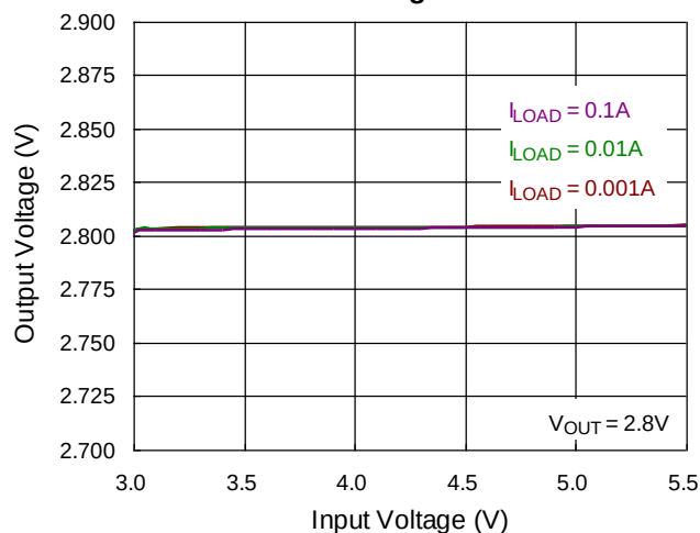
Line Regulation
