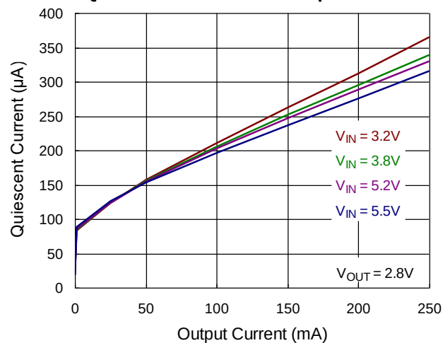
Quiescent Current vs. Output Current
