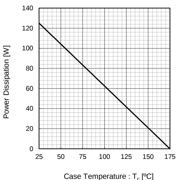
Fig.6 Power Dissipation
