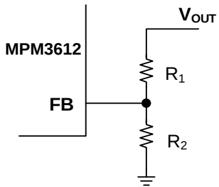
Figure 4: Feedback Network
