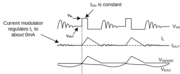
Figure 3: Light-Load Operation
