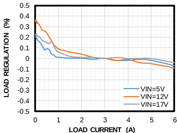
Load Regulation
