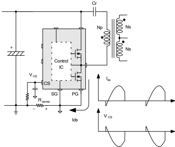
Figure 23. Half-Wave Sensing
