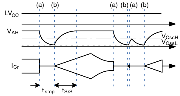
Figure 21. Self Auto-Restart Operation
