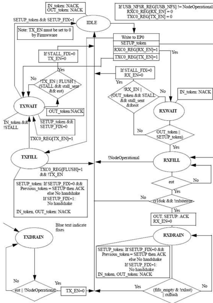
Figure 99. Endpoint 0 operation
