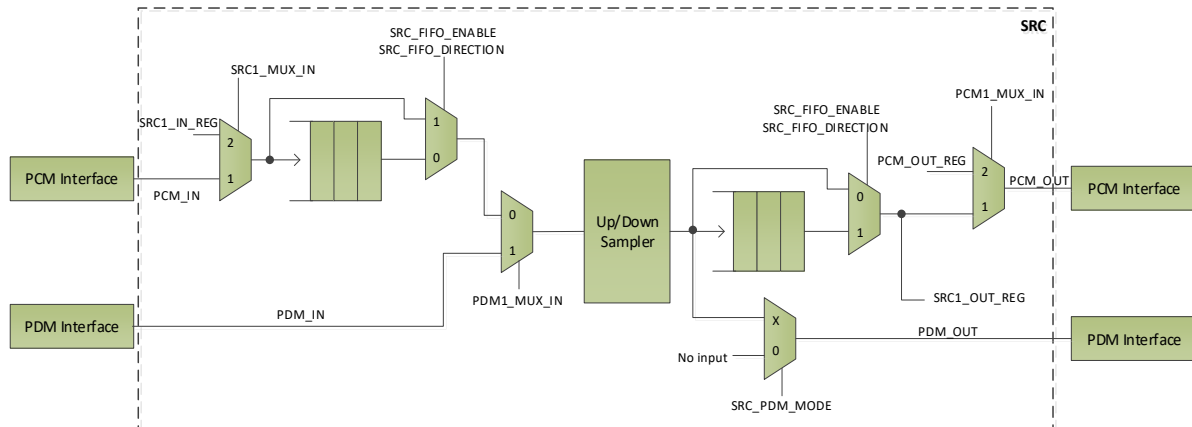
Figure 63. Audio unit block diagram
