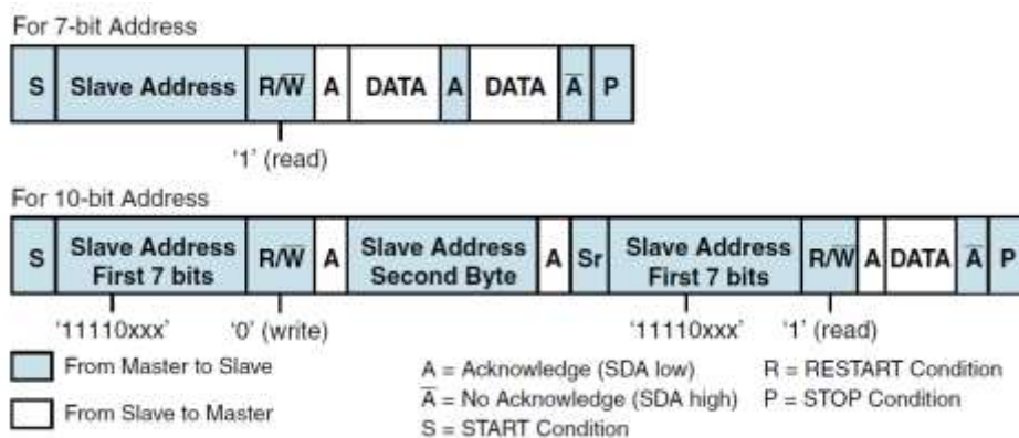
Figure 76. Master-Receiver protocol
