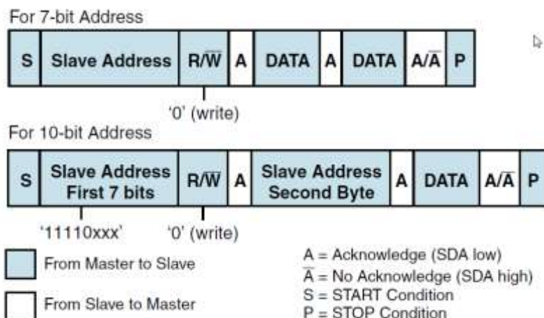
Figure 75. Master-Transmitter protocol
