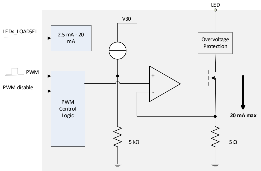
Figure 107. LED Driver block diagram
