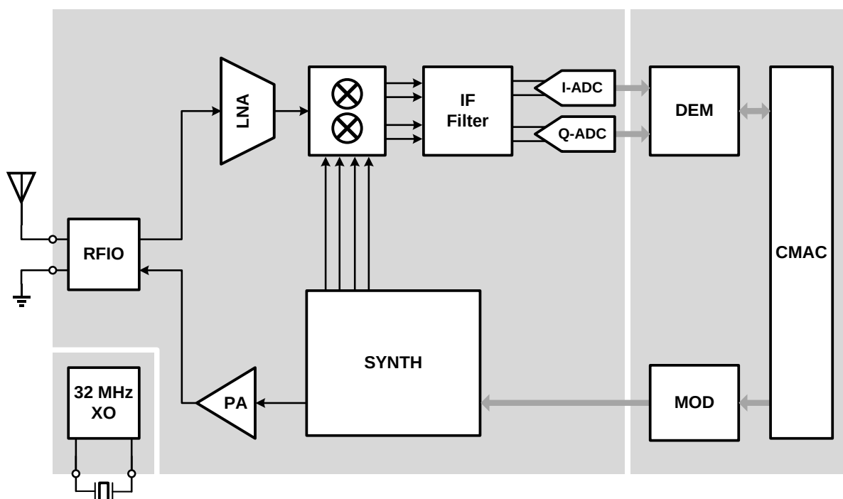
Figure 111. Radio block diagram
