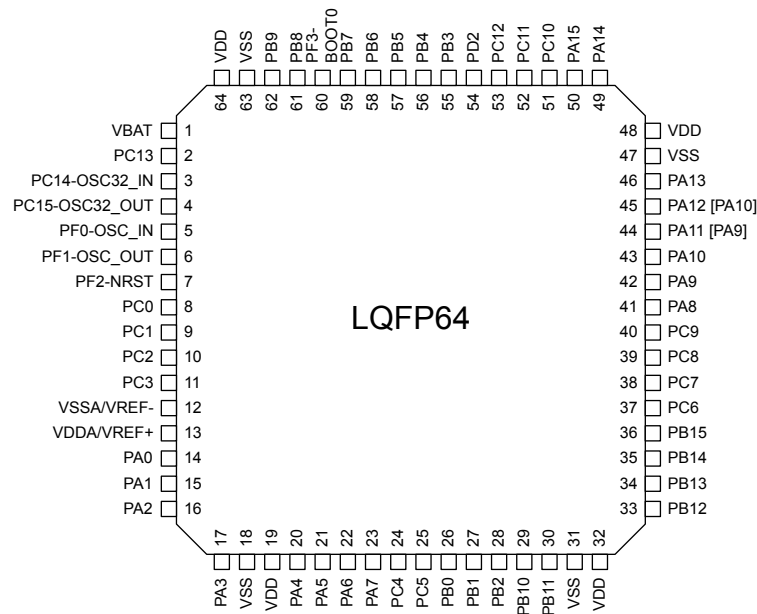
Figure 8. LQFP64 pinout
