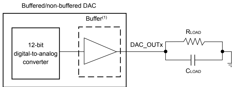
Figure 26. 12-bit buffered / non-buffered DAC
