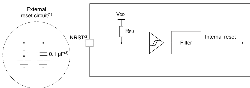
Figure 23. Recommended NRST pin protection
