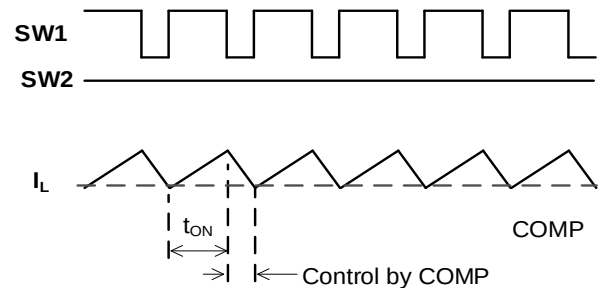
Figure 4: Buck Waveform
