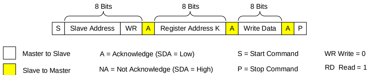
Figure 11: I 2 C Write Example (Write Single Register)
