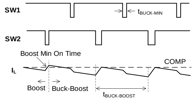
Figure 7: Buck-Boost Waveform
