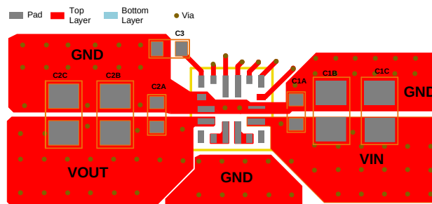
Figure 16: Recommended PCB Layout (Top)
