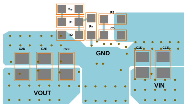
Figure 17: Recommended PCB Layout (Bottom)
