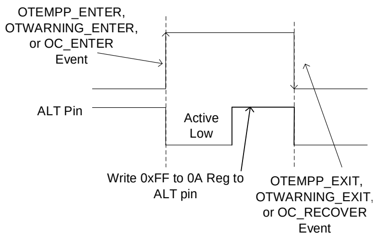
Figure 14: ALT Behavior during OTP, OTW, and OC Recovery
