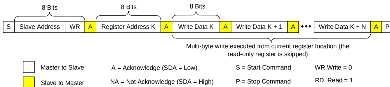
Figure 12: I²C Write Example (Write Multi-Register)
