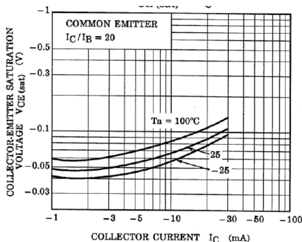
Fig. 10.22 RN2304 V_{CE(sat)}-I_C
