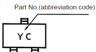
Fig. 9.3 Marking RN2303
