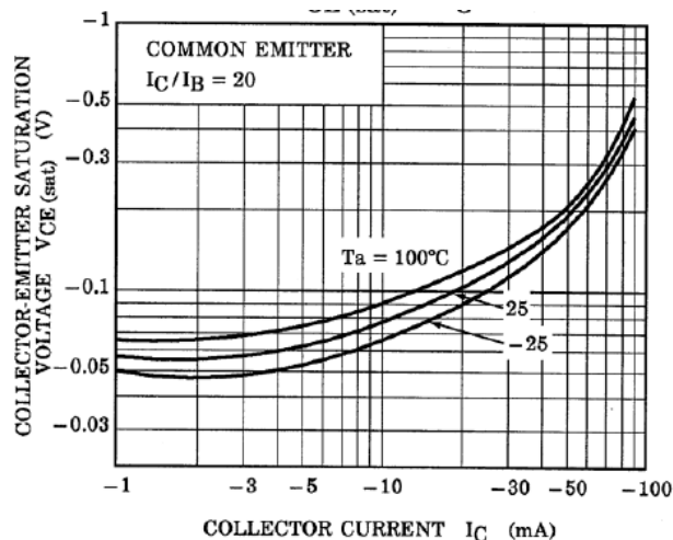
Fig. 10.23 RN2305 V_{CE(sat)}-I_C
