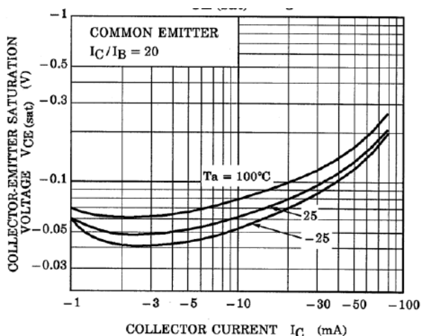
Fig. 10.21 RN2303 V_{CE(sat)}-I_C
