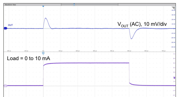
Load = 0 to 10 mA, C OUT = 10 µF
