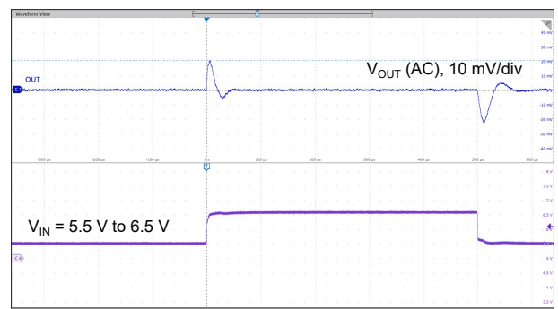
V IN = 5.5 V to 6.5 V, C OUT = 10 µF
