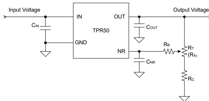
Figure 20. Output Voltage Trim with NR/TR Pin
