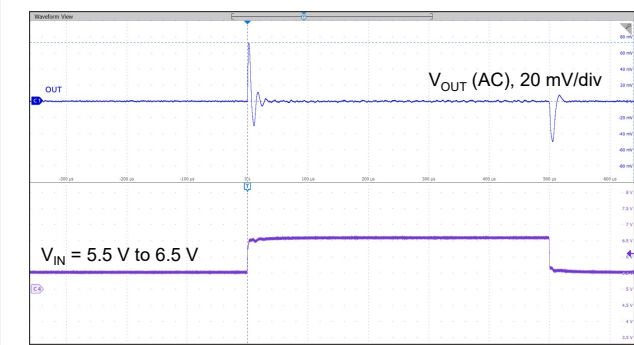
V IN = 5.5 V to 6.5 V, C OUT = 1 µF
