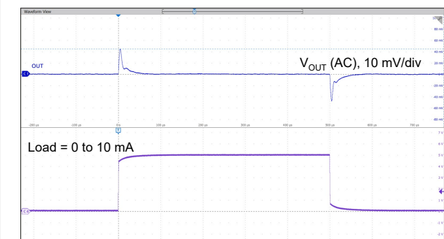
Load = 0 to 10 mA, C OUT = 1 µF
