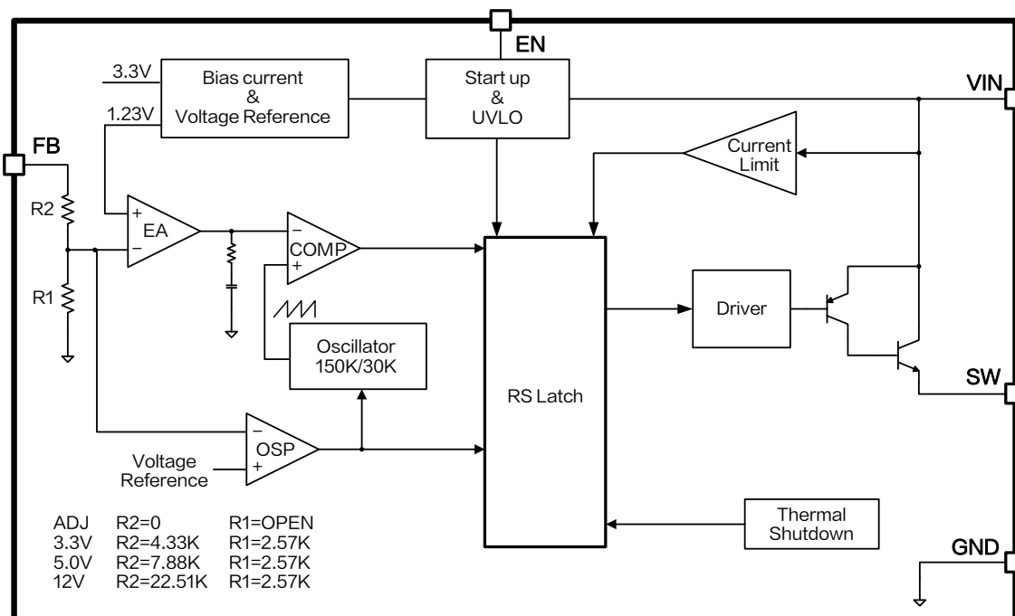
Figure3. Function Block Diagram of XL2596HVP
