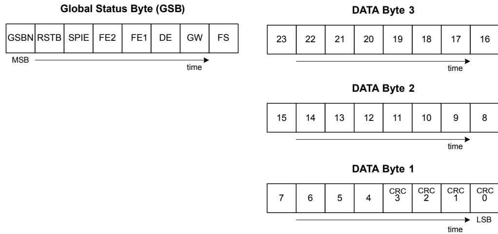
Figure 35. SDO frame
