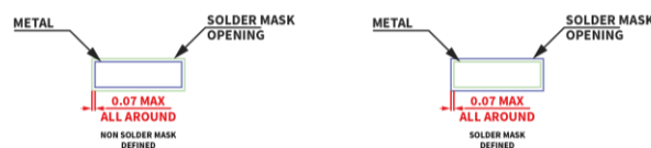
Figure 9.8 SOP16(600mil)/SOWW16 Package Board Layout Example
