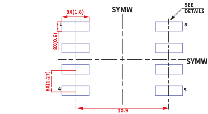
LAND PATTERN EXAMPLE(mm) 9.1mm NOMINAL CLEARANCE/CREEPAGE
