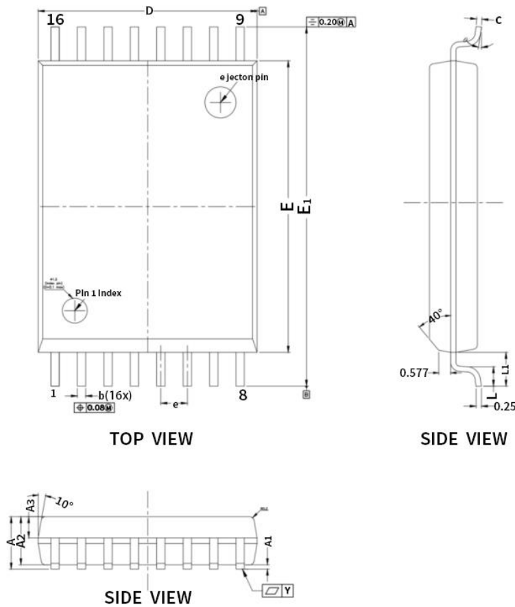
Figure 9.7 SOP16(600mil)/SOWW16 Package Shape and Dimension in millimeters
