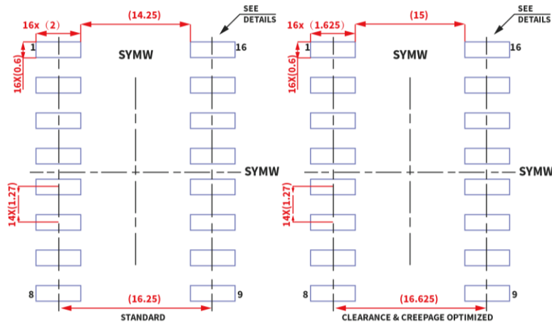
Figure 9.7 SOP16(600mil)/SOWW16 Package Shape and Dimension in millimeters
