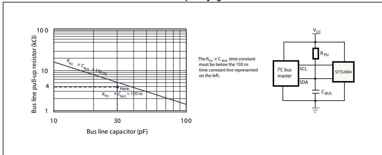
Figure 20. Pull-up resistor values versus bus line capacitance
