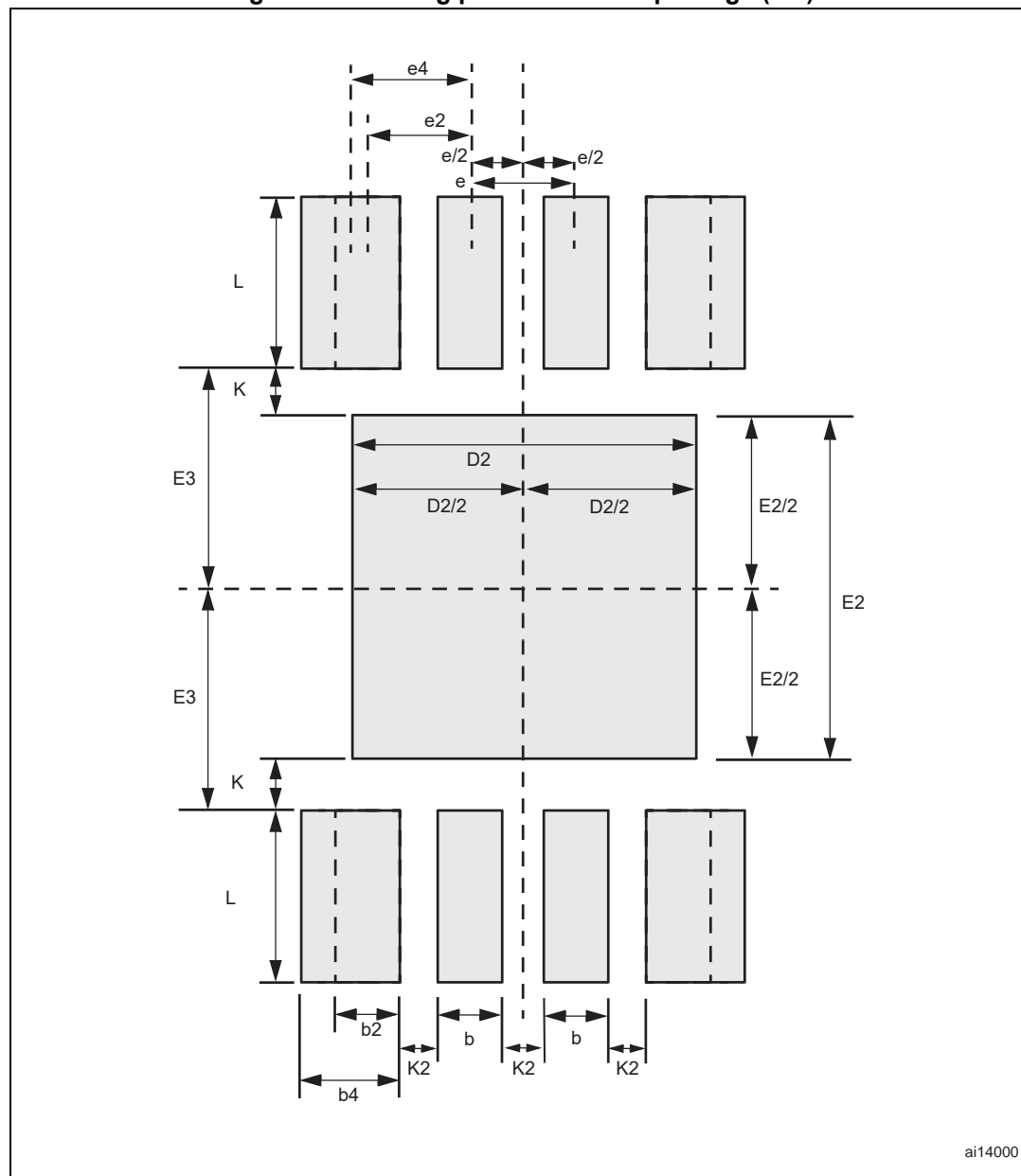
Figure 23. Landing pattern - TDFN8 package (DN)
