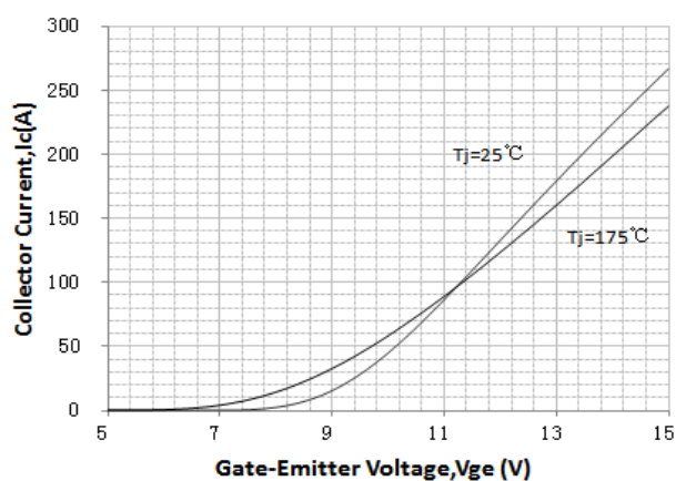
Transfer Characteristics
