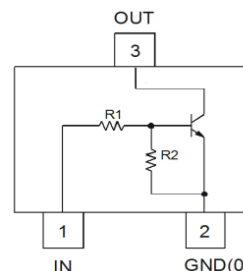
Device Schematic
