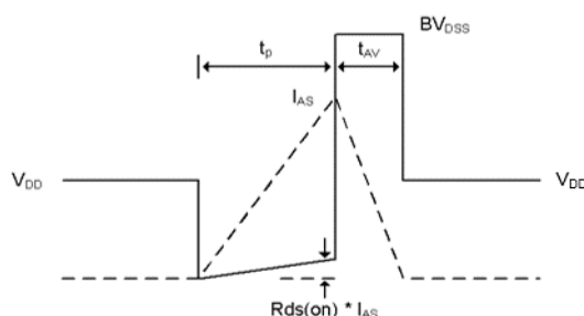
Fig18-2. Unclamped inductive waveform
