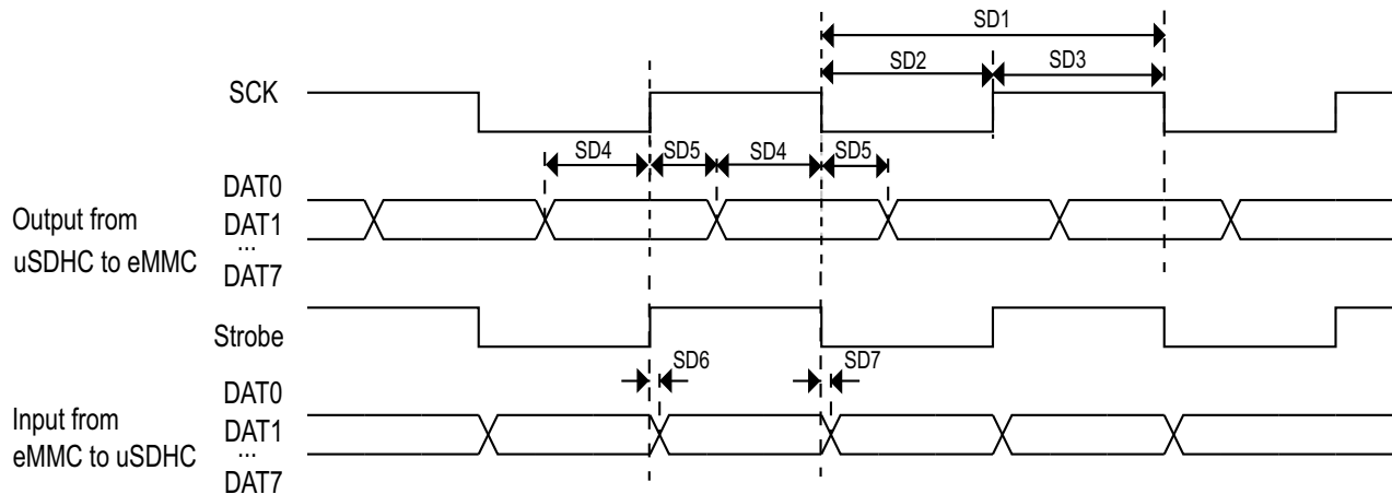
Figure 24. HS400 timing
