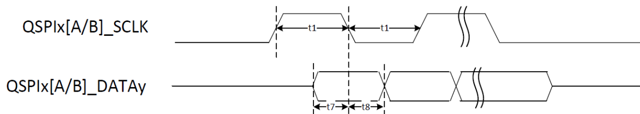
Figure 45. FlexSPI read timing diagram (DDR mode)
