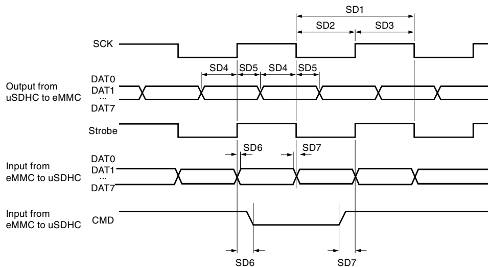
Figure 30. HS400 timing
