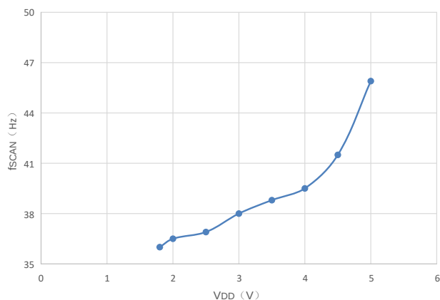
扫描频率 vs. V_{DD}
