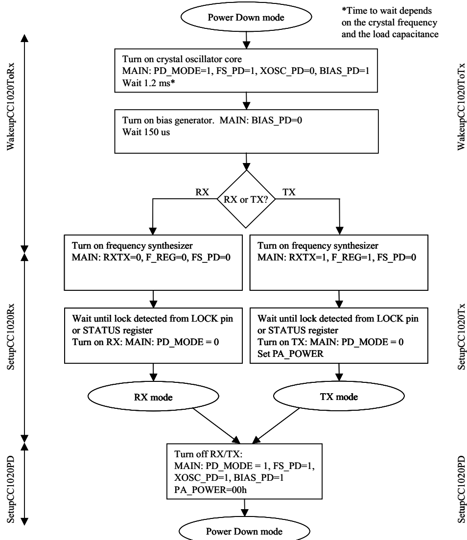
Figure 5-28. Sequence for Activating RX or TX Mode
