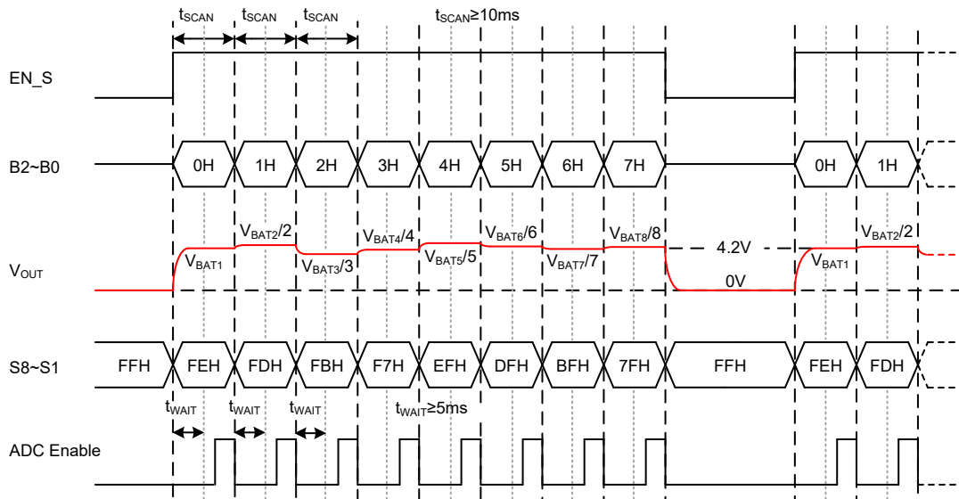
8S Battery Monitoring Timing
