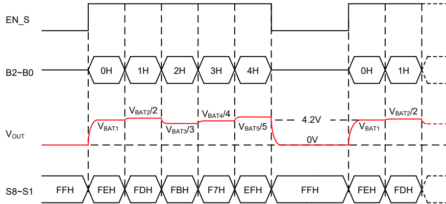
5S Battery Monitoring Timing
