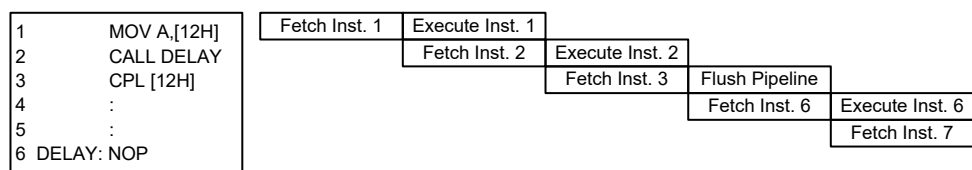
Instruction Fetching
