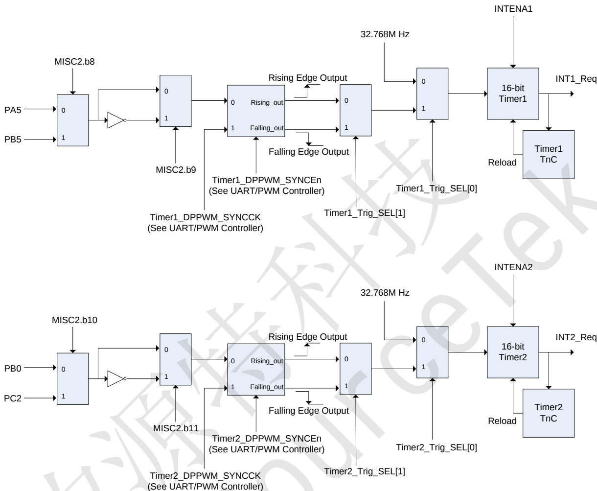
Figure 7.2 Timer1&Timer2 Structure
