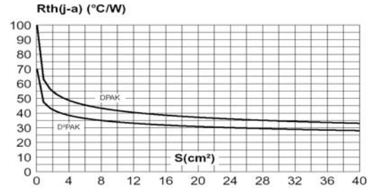
Fig. 10: DPAK and D 2 PAK Thermal resistance junction to ambient versus copper surface under tab (printed circuit board FR4, copper thickness: 35 μm).
