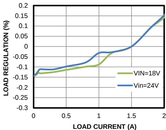
Load Regulation
