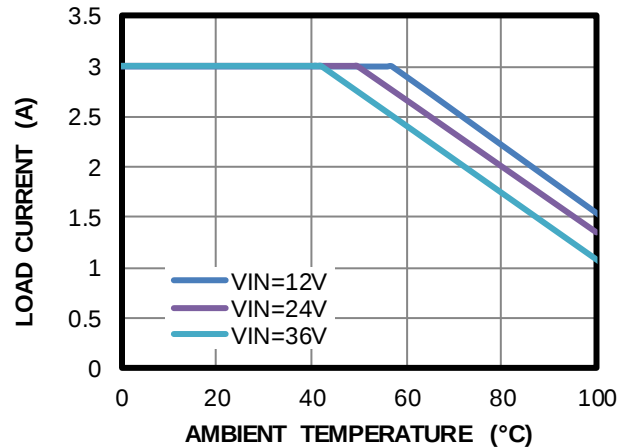
Thermal Derating
