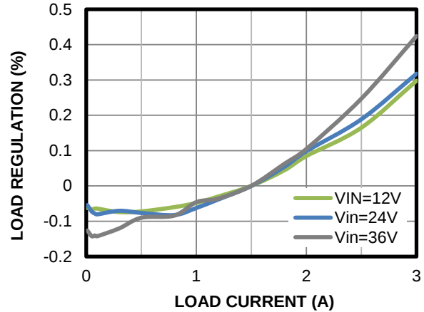
Load Regulation
