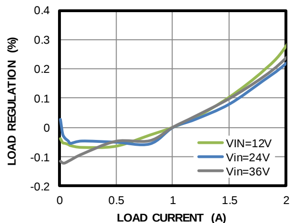
Load Regulation
