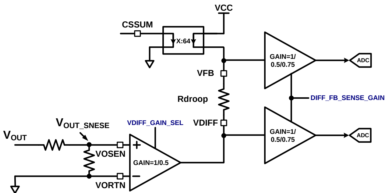
Figure 21: DC Loop Gain Selection Block Diagram
