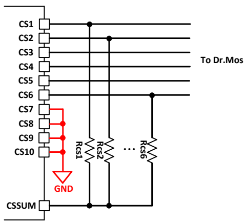
Figure 15: CS Pins Program to 6-Phase
