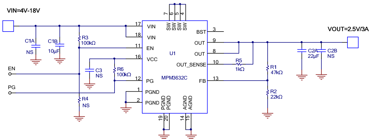
Figure 10: 2.5V Output
