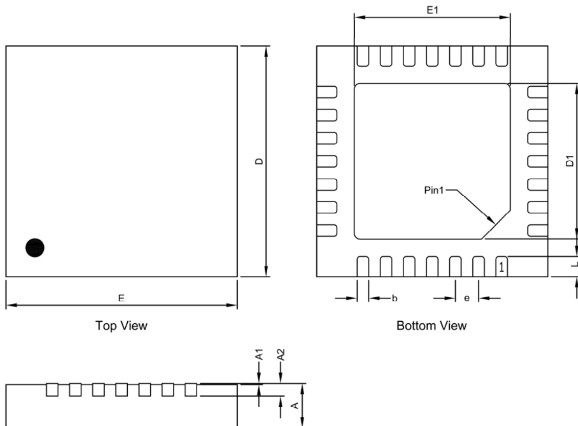
TQFN4X4-28 Package
