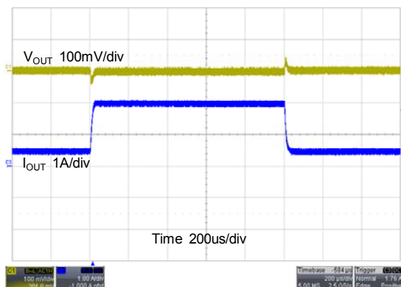
CH2, Fsw=1.5MHz, Iout=500mA~2A, VIN=4.2V
