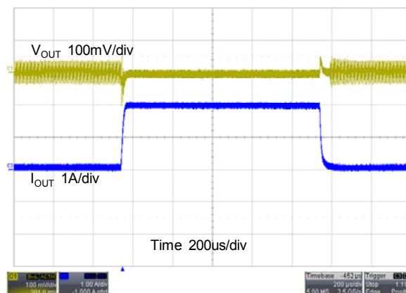
CH2, Fsw=1.5MHz, Iout=100mA~2A, VIN=4.2V
