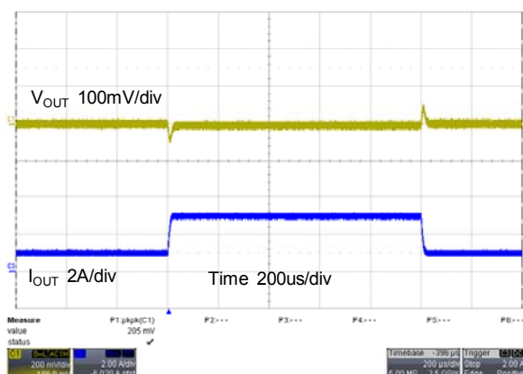
CH3, Fsw=1.5MHz, Iout=500mA~3A, VIN=4.2V
