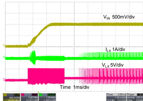
CH1 VIN=3.6V, Vout=1.0V, Iout=30mA (PSM)
