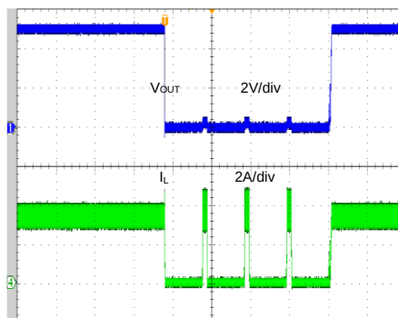
Short Circuit Protection ( V_{IN}=12V , V_{OUT}=5V , 3.5A to Short)
