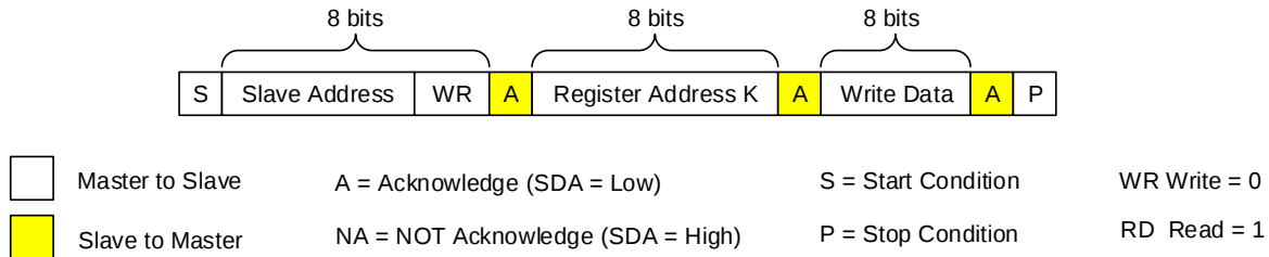
Figure 14a: I 2 C Write Example – Write Single Register
