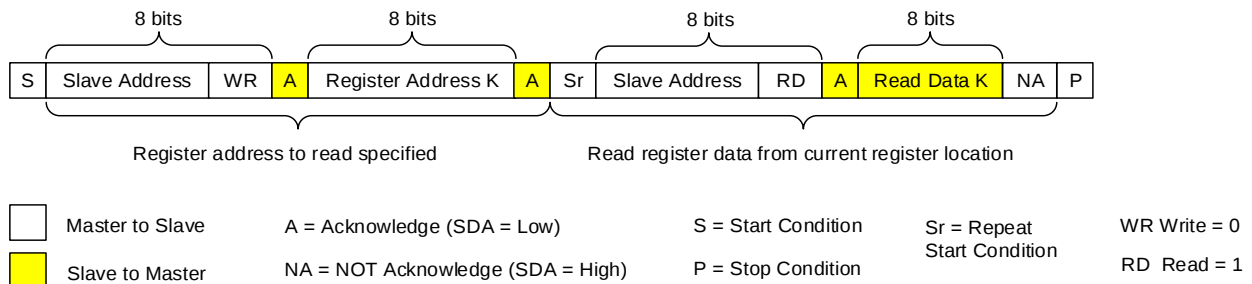
Figure 14c: I 2 C Read Example – Read Single Register
