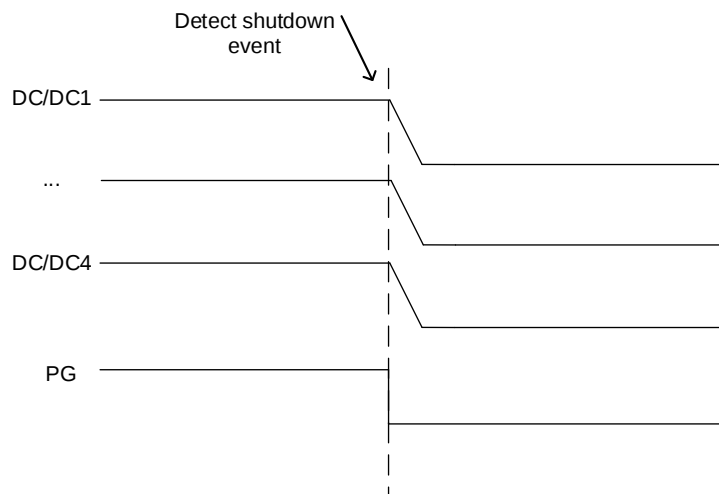
Figure 10: Shutdown Sequence
