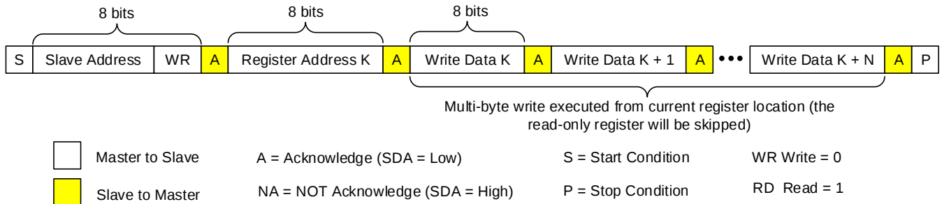
Figure 14b: I 2 C Write Example – Write Multi-Register
