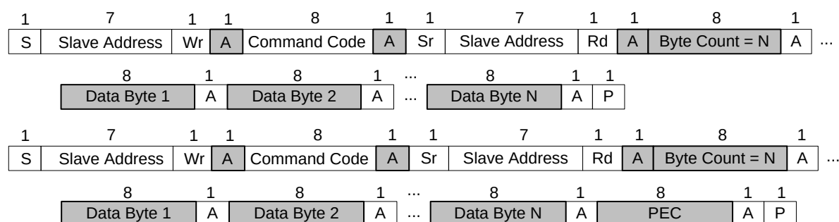
Figure 5: PMBus Message Format
