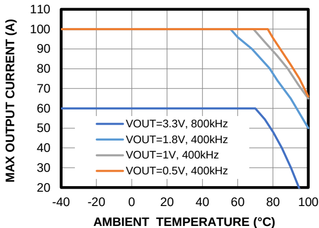
Thermal Derating
