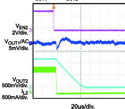
CH1 Steady State, CH2 EN Off
