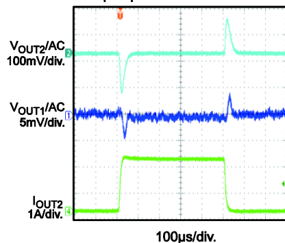
CH1 Steady State, CH2 Load Transient
