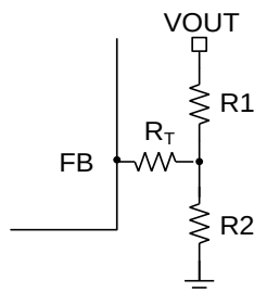
Figure 5: T-Type Feedback Network
