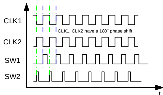
Figure 2: 180° Out-of-Phase Operation
