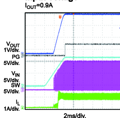
Start-Up through Input Voltage I_{OUT}=0.9A
