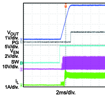
Start-Up through EN/SYNC I_{OUT}=0.9A
