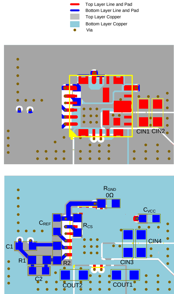
Figure 7: Recommended PCB Layout
