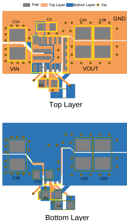
Figure 6: Recommended PCB Layout
