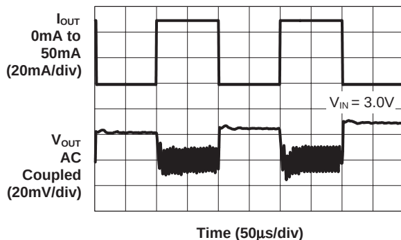
Load Transient Response for 50mA
