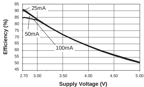
Efficiency vs. Supply Voltage
