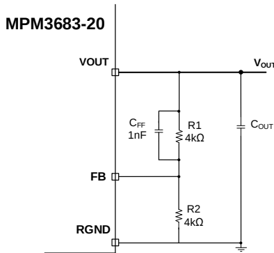
Figure 6: Circuit Connection
