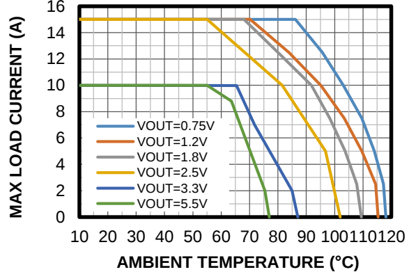
Thermal Derating
