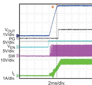
Start-Up through EN/SYNC I_{OUT}=1.5A
