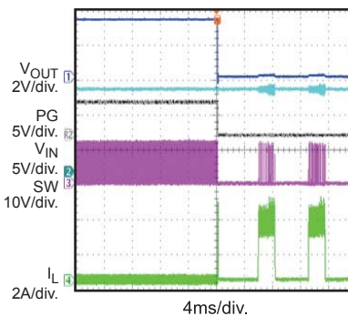
SCP Entry I_{OUT}=0A
