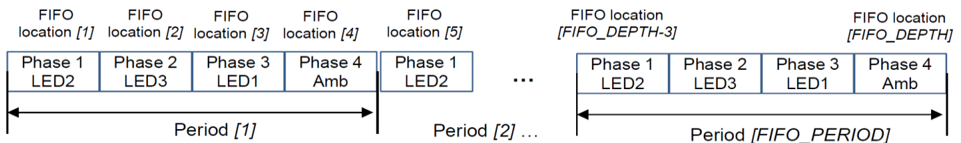
Figure 14. Scheme for FIFO write for the case where 4 phases of data are selected to be stored
