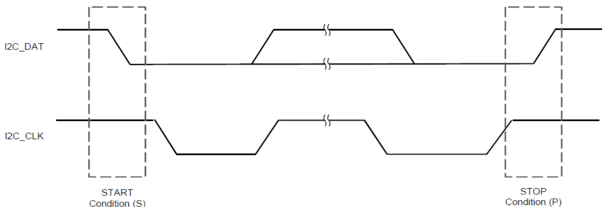
Figure 30. Transition of I2C_DAT during Start and Stop Conditions
