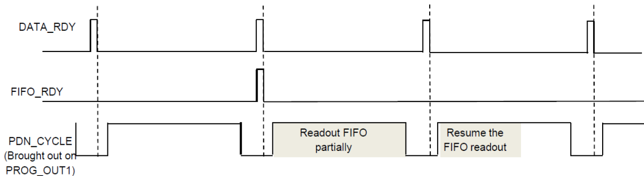
Figure 24. FIFO readout over multiple PDN_CYCLE phases
