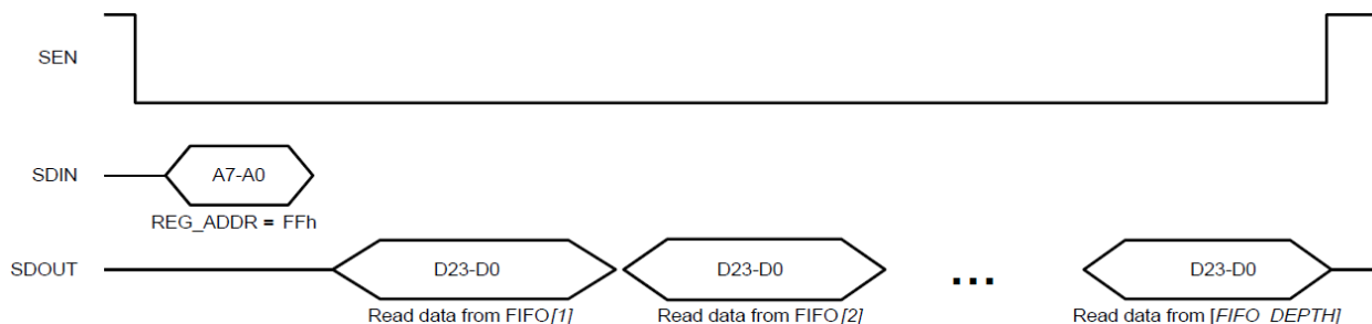
Figure 41. Continuous FIFO readout through the SPI interface
