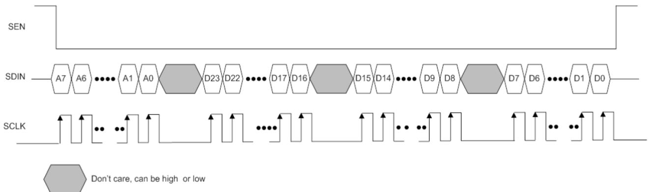
Figure 37. PPSI262 SPI write timing diagram
