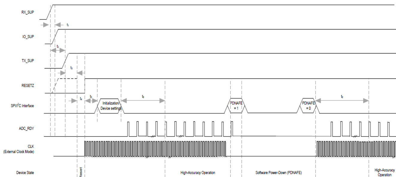
Figure 58. Power Supply Sequencing, Device Initialization, and Software Powerdown Timing
