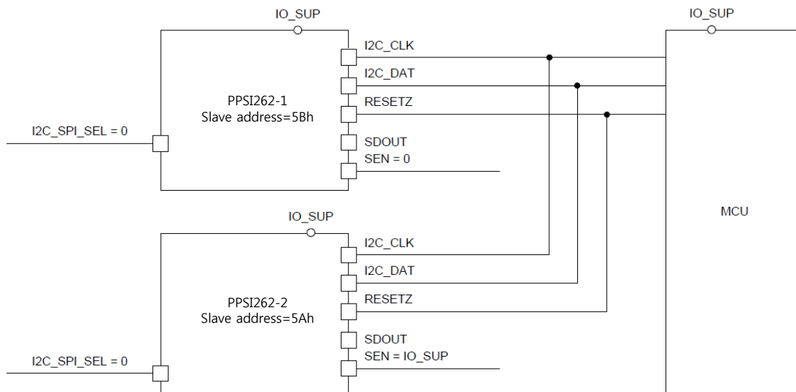
Figure 54. Connection of two PPSI262s to the MCU when operating in I 2 C mode
