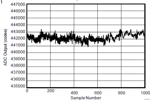
Figure 50. (LED-Ambient) data with Optimal AFE setting
