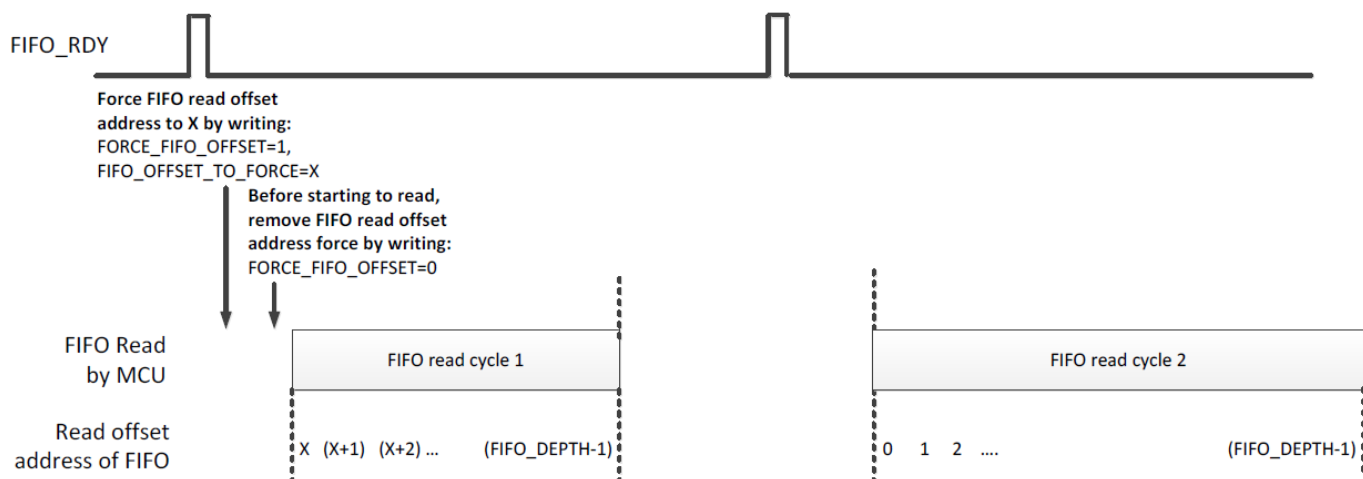
Figure 19. Recommended Method to Deassert FORCE_FIFO_OFFSET When Using a Single Read Burst to Read the FIFO
