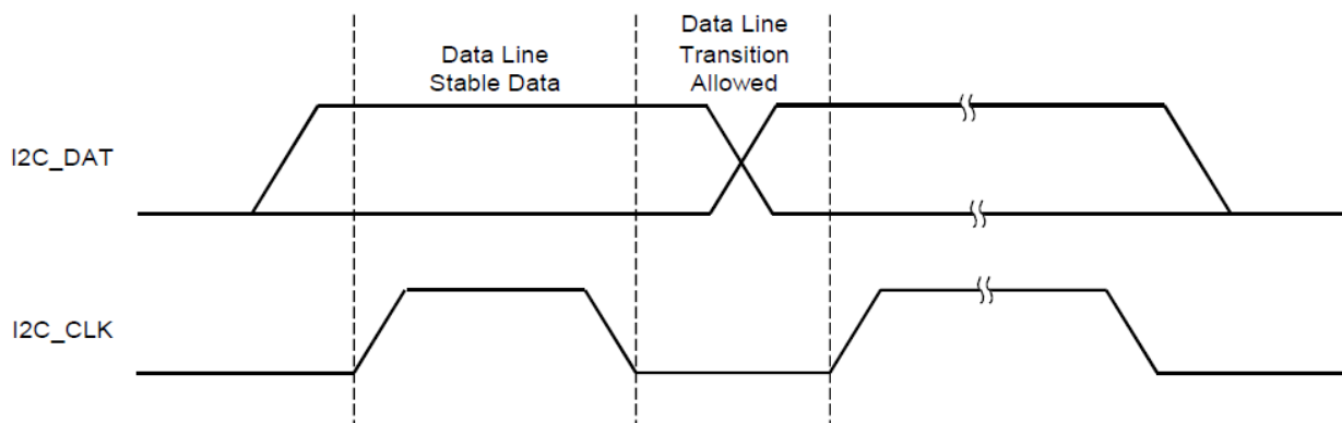
Figure 29. Allowed Transition of I2C_DAT while Transmission of Data Bits
