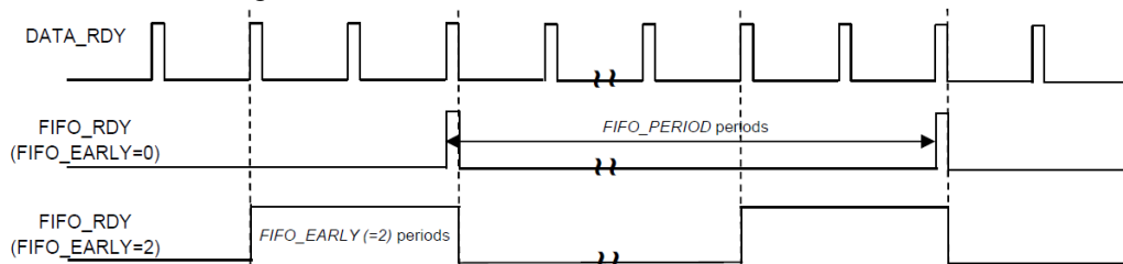
Figure 15. Scheme for FIFO_RDY generation for FIFO_EARLY=0 and FIFO_EARLY=2
