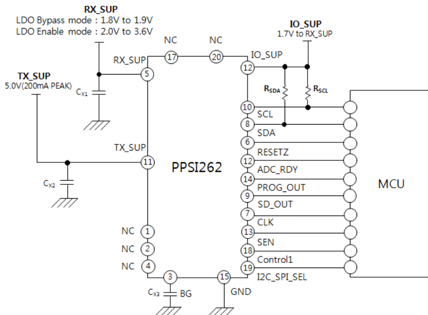
Figure 43. Hardware pin connection diagram in external clock mode
