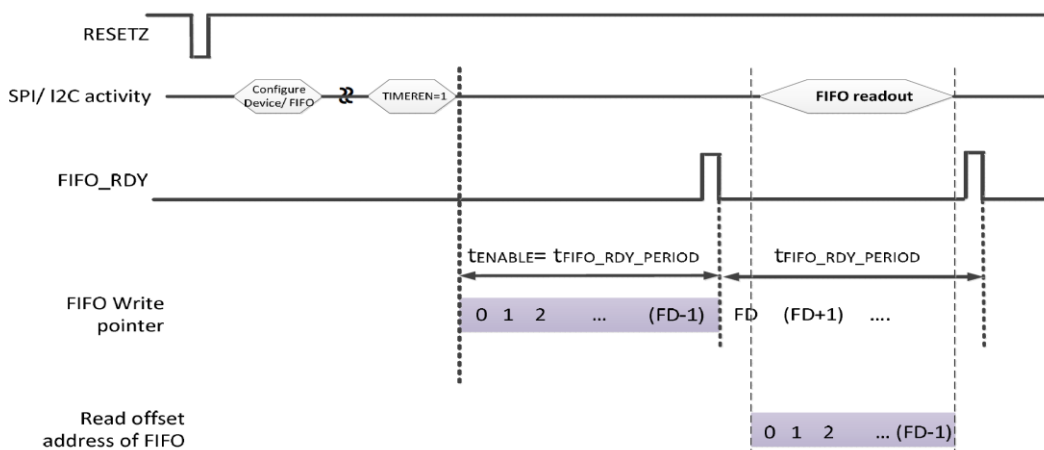
Figure 21. Recommended scheme to enable the FIFO the first time after reset
