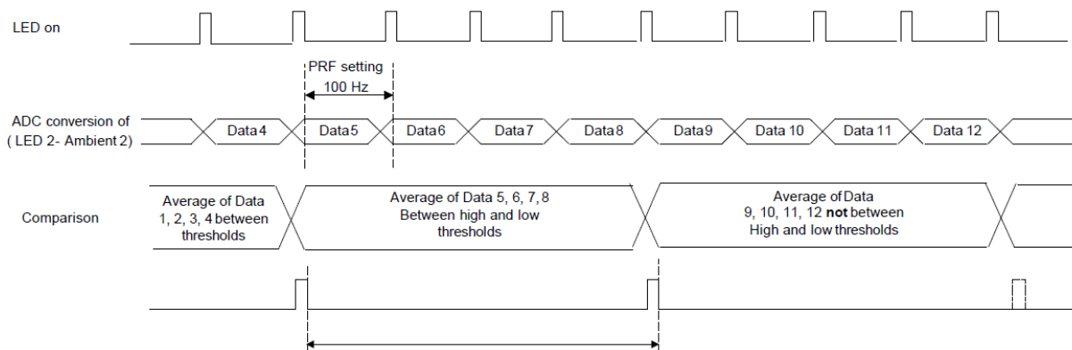
Figure 28. THR_DET_RDY Interrupt Generation Timing Diagram
