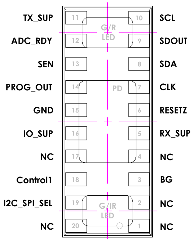
Figure 2. PKG Diagram.
