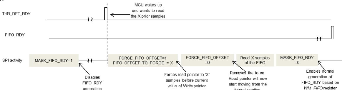
Figure 26. Method of resuming FIFO read following a FIFO_RDY masking phase
