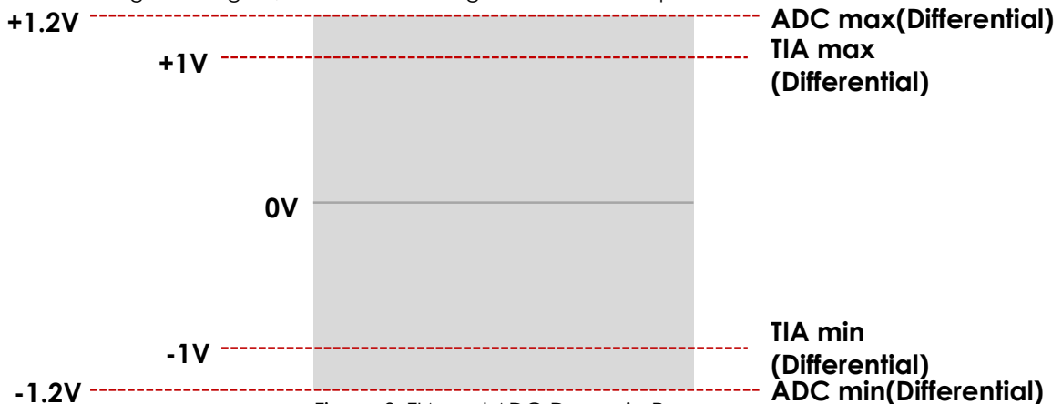
Figure 9. TIA and ADC Dynamic Ranges
