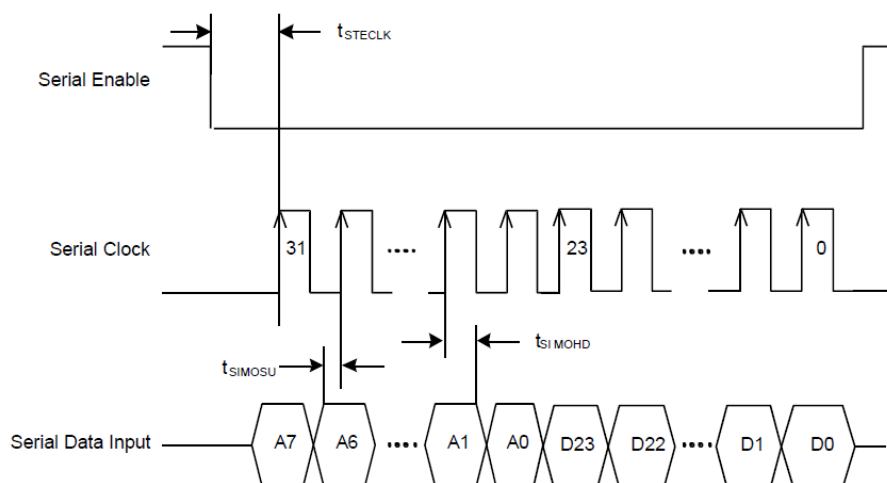
Figure 2. Serial Interface Timing Diagram, Write Operation
