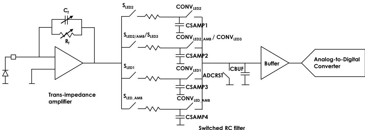
Figure 8. Illustration of the noise reduction filter
