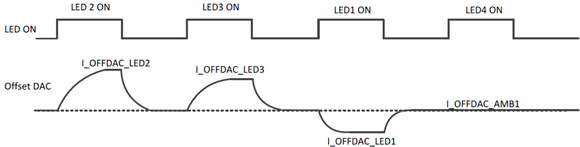
Figure 7. Transitions of the offset DAC when EARLY_OFFSET_DAC is set to '1'
