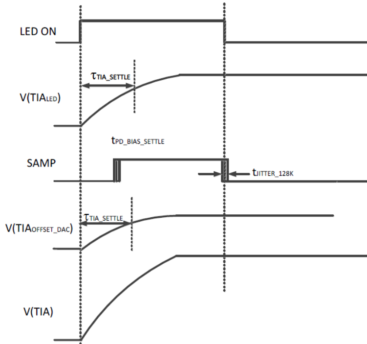
Figure 52. TIA settling transient with EARLY_OFFSET_DAC set to '1'
