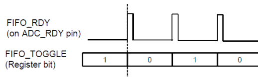
Figure 16. Update of FIFO_TOGGLE register bit
