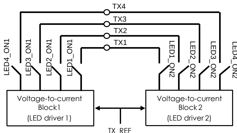
Figure 10. Support of parallel LED drive
