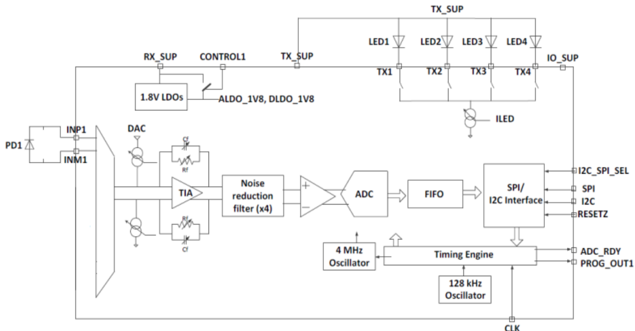
Figure 1. Block Diagram.
