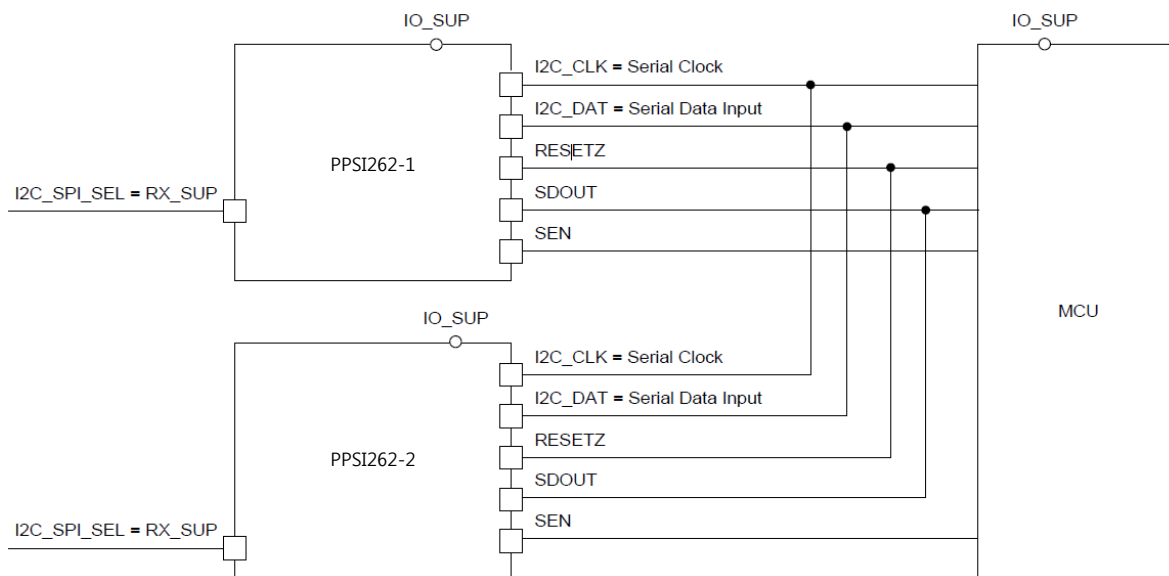
Figure 56. Connection of two PPSI262s in SPI mode that share a portion of SPI bus
