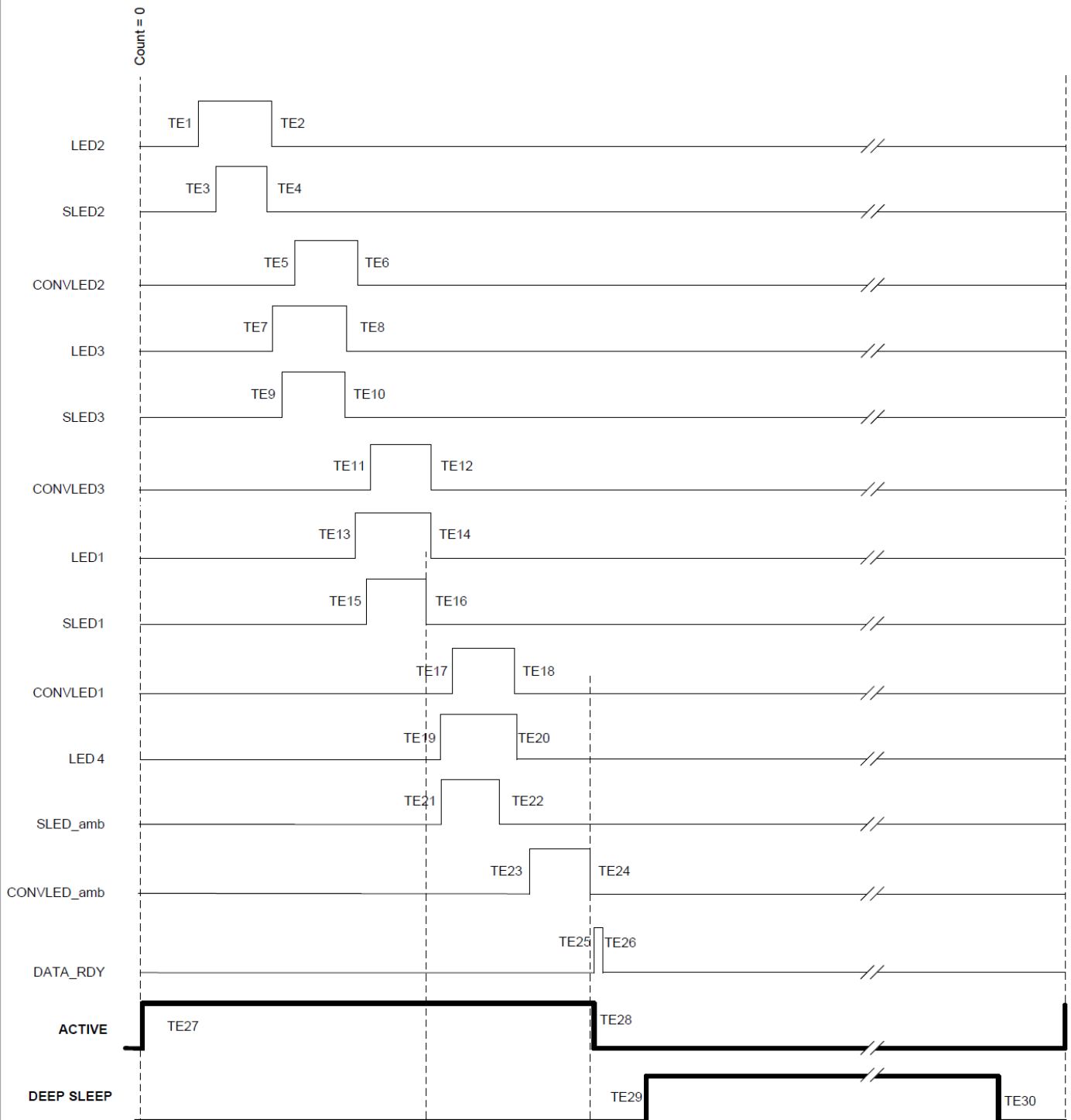
Figure 13. Timing Diagram of various programmable signal phases
