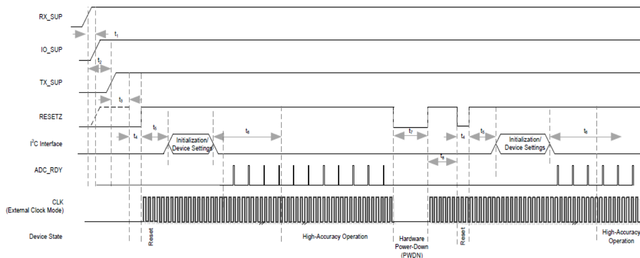
Figure 57. Power Supply Sequencing, Device Initialization, and Hardware Powerdown Timing
