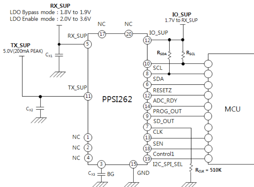
Figure 44. Hardware pin connection diagram in internal oscillator mode
