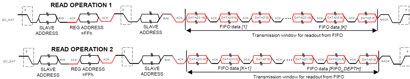
Figure 36. I 2 C Readout from FIFO over two read operations
