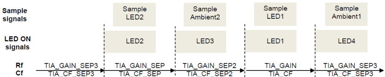
Figure 4. TIA R_f , C_f transitions within a period for ENSEPGAIN4=1
