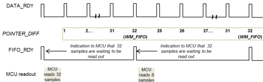
Figure 25. FIFO mode based on programmable watermark level
