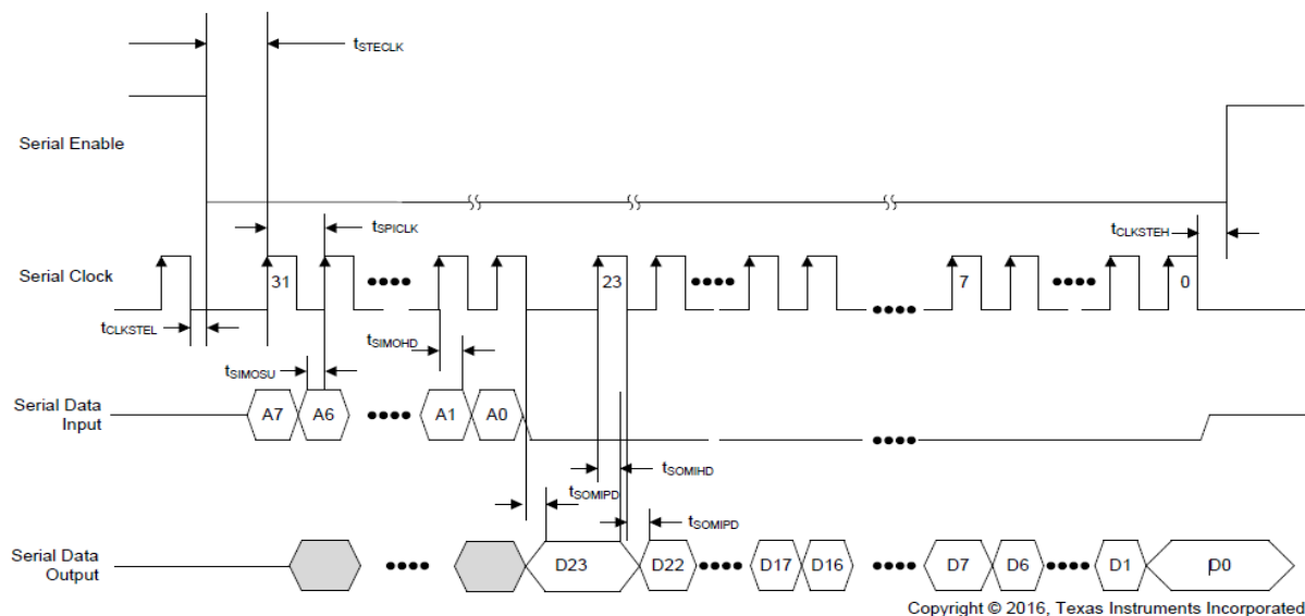
Figure 1. Serial Interface Timing Diagram, Read Operation
