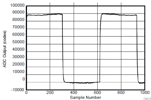
Figure 48. Ambient data with ambient light modulation
