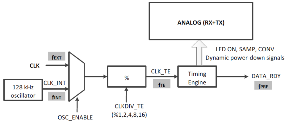
Figure 12. Clocking scheme
