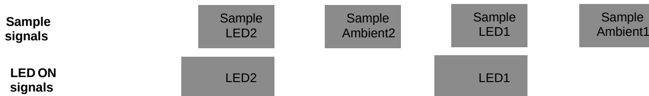
Figure 46. Use Case with Two LEDs and Two Ambient Phases
