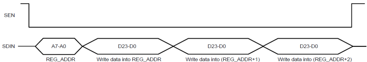
Figure 39. Continuous SPI write (RW_CONT = 1)
