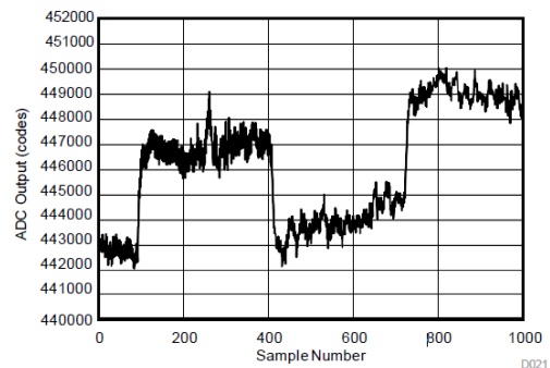
Figure 49. (LED-Ambient) data with Non-Optimal AFE setting
