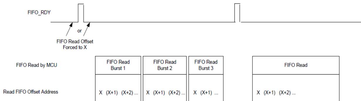
Figure 18. Read Offset Address of the FIFO When FORCE_FIFO_OFFSET is Enabled
