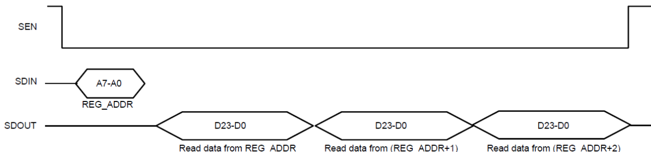
Figure 40. Continuous SPI read (RW_CONT = 1, SPI_REG_READ = 1)
