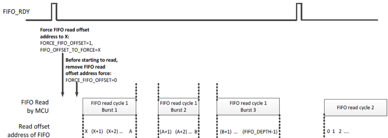
Figure 20. Recommended Method to Deassert FORCE_FIFO_OFFSET When Using Multiple Read Bursts to Read the FIFO
