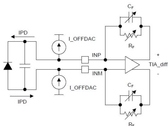
Figure 5. Offset Cancellation Current Polarity Diagram
