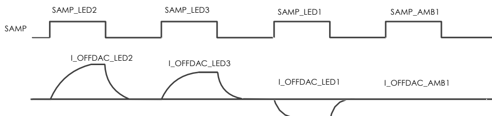
Figure 6. Transitions of the offset DAC at the SAMP phases
