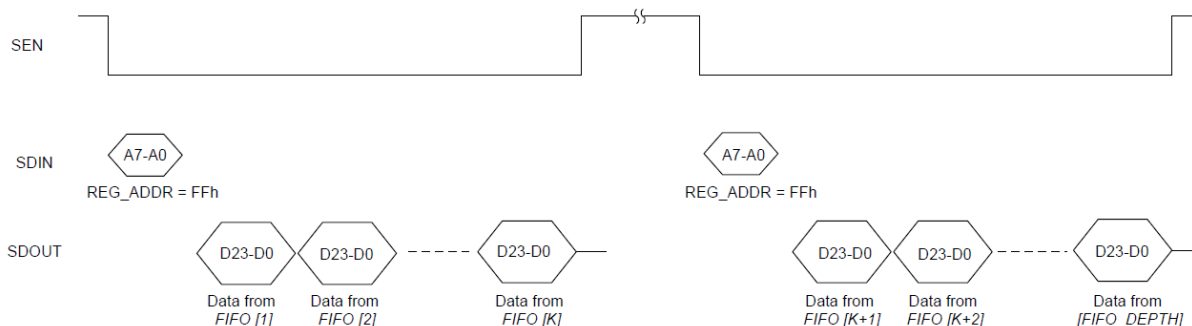
Figure 42. FIFO readout over two read operation
