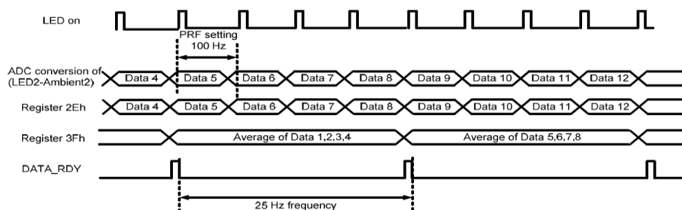
Figure 27. Decimation mode Timing diagram (Decimation factor=4, PRF=100Hz)
