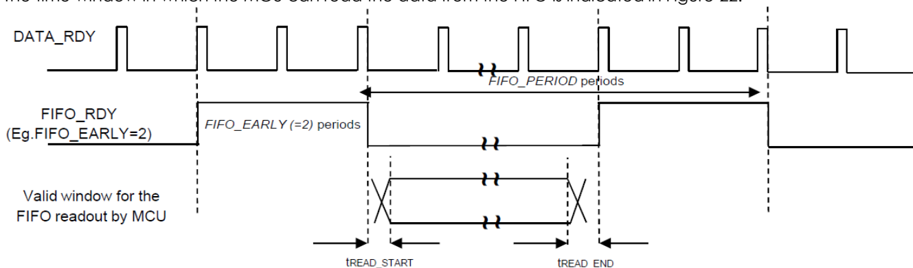
Figure 22. Time window for the MCU to read the FIFO
