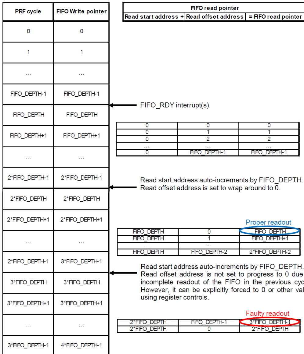
Figure 17. Progression of FIFO read and write pointer
