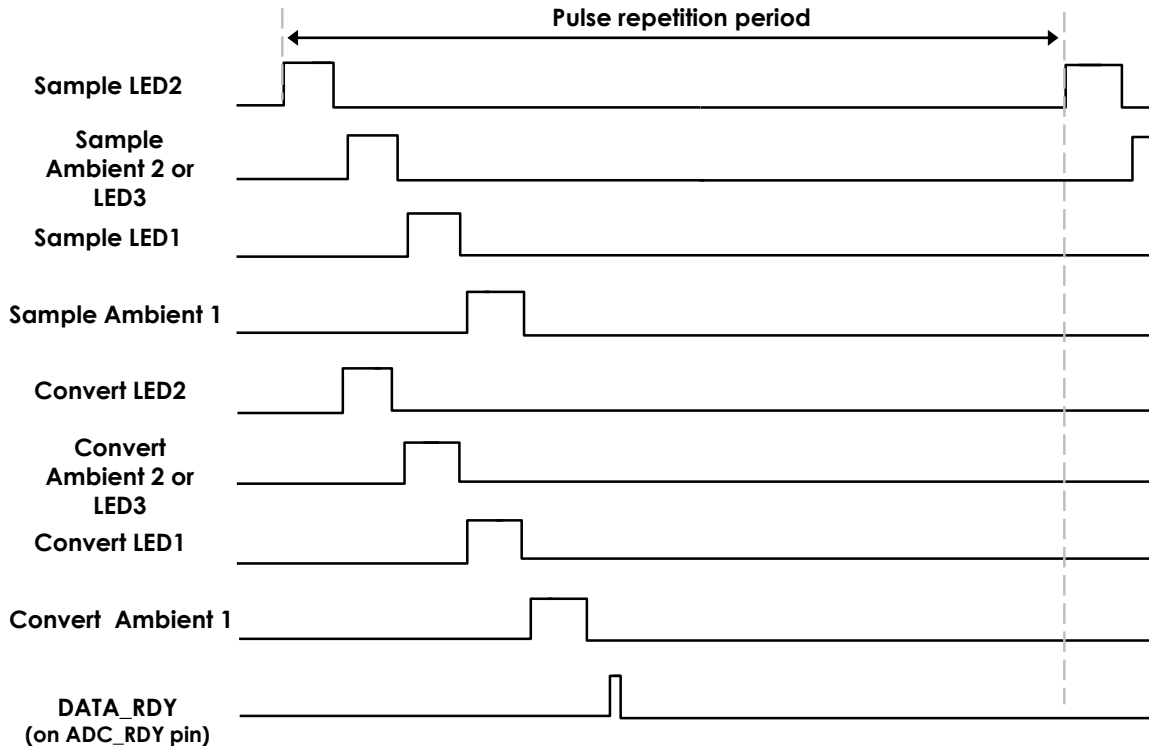
Figure 3. Sequence of Four Sampling and Conversion Phases
