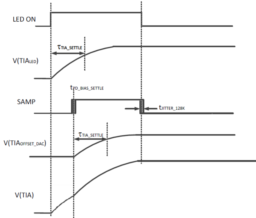
Figure 51. TIA settling transient
