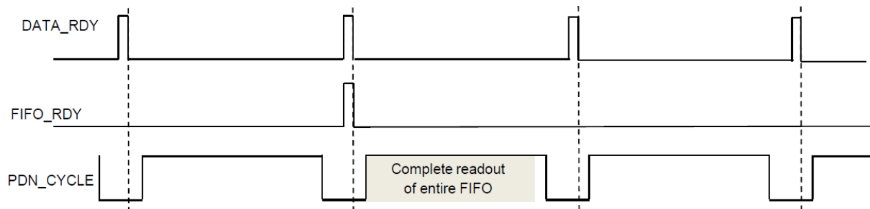
Figure 23. Time window for the MCU to read the FIFO
