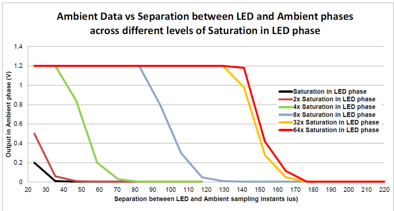
Figure 53. Recovery of the ambient phase as a function of the over-saturation factor in the LED phase
