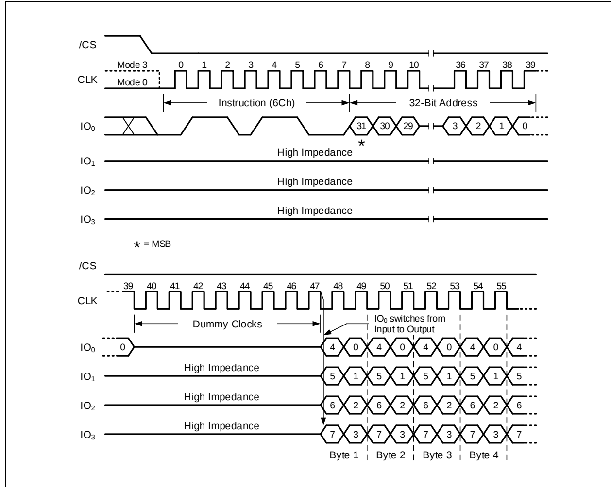
Figure 22. Fast Read Quad Output with 4-Byte Address Instruction
