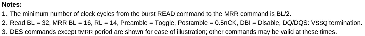
Figure 78 - READ to MRR Timing
