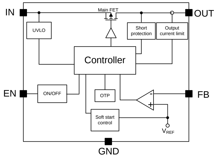
Figure 2. Block Diagram
