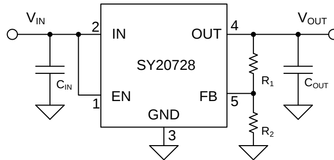
Figure 1. Adjustable Output Regulator
