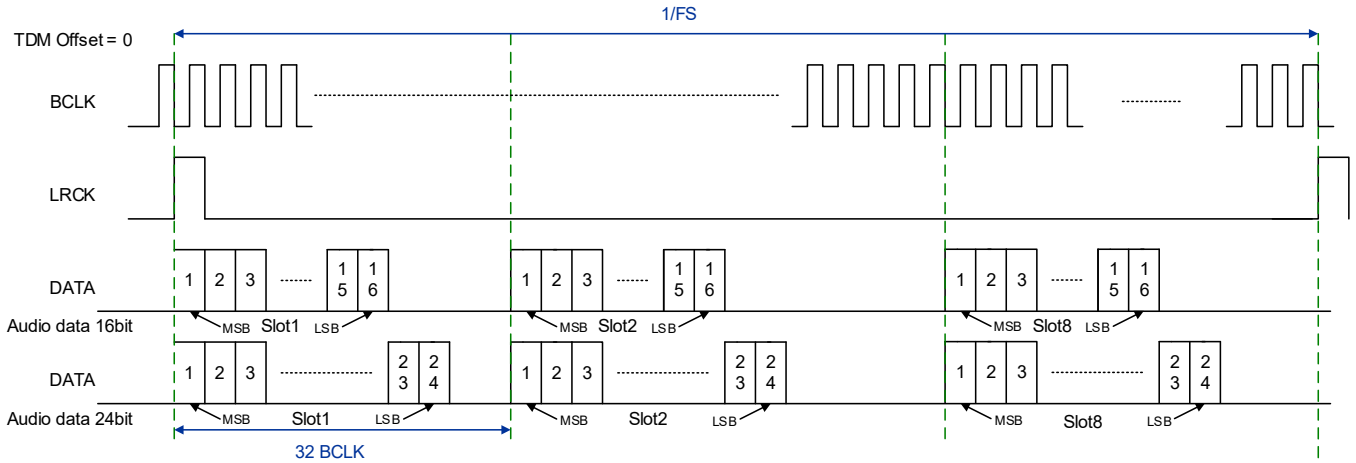
Figure 8. TDM (Offset = 0)
