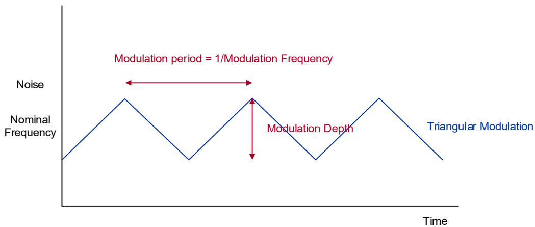
Figure 16. Spread-Spectrum Algorithm
