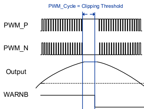
Figure 18. Clip Detection
