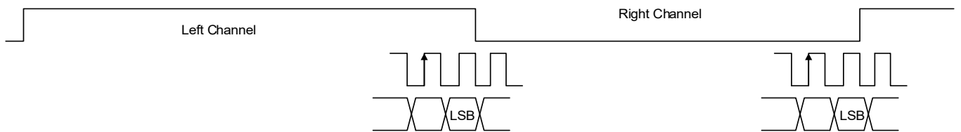
Figure 6. Right-Justified
