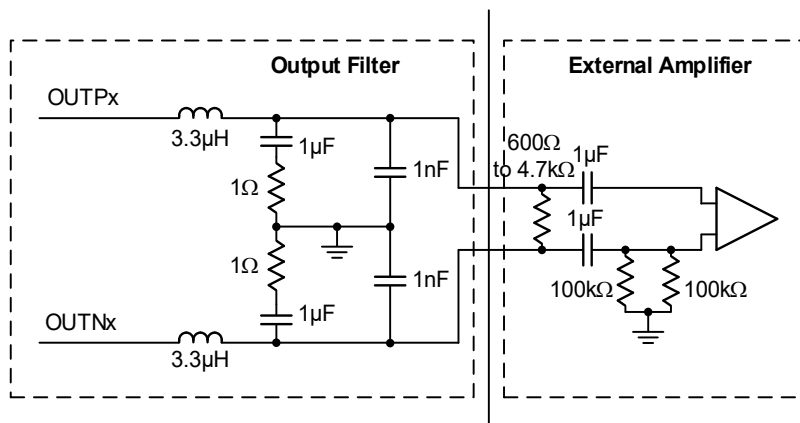
Figure 19. Output Filter
