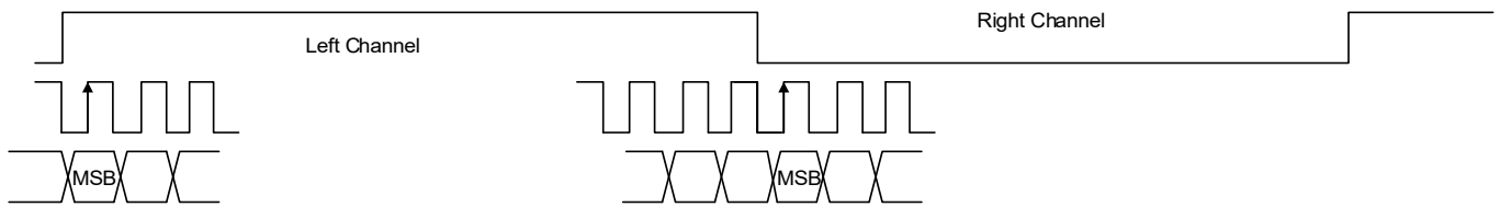
Figure 5. Left-Justified
