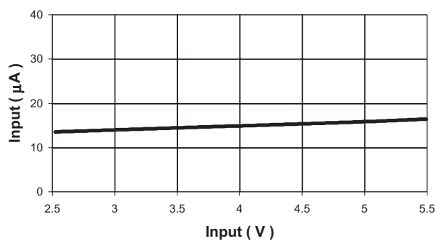
Quiescent Current
