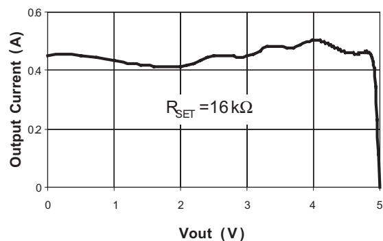
Output Current vs V_{OUT}
