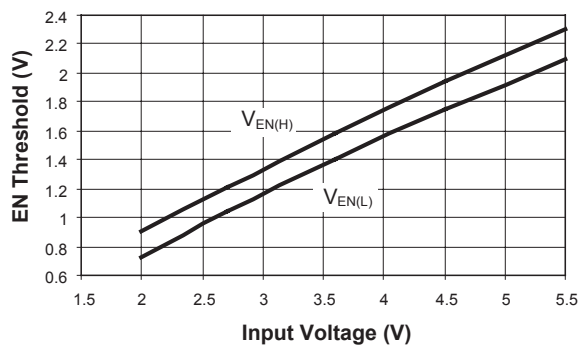
Typical EN Threshold vs. Input Voltage
