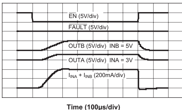
Turn-On/Off Response with 20\Omega 1\mu\text{F} Loads
